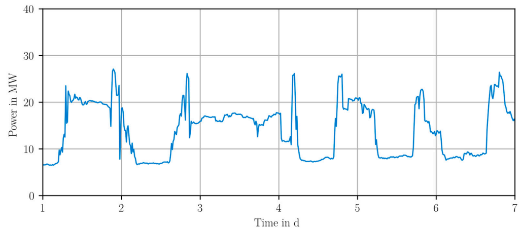
Figure 2. Measured load profile of the vessel propulsion load and hotel load for seven days during summer.
