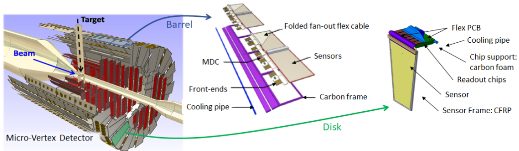
Figure 1. Micro-Vertex Detector (left), barrel and disk detector modules (right).
