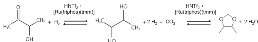
Fig. 5 Reaction scheme towards 4,5-dimethyl-1,3-dioxolane. Hydrogenation of acetoin to 2,3-BDO catalyzed by the [Ru(triphos)(tmm)] catalyst at 90 °C and 100 bar. Further, a transformation of 2,3-BDO, CO 2 , and H 2 to 4,5-dimethyl-1,3-dioxolane catalysed by the same [Ru(triphos)(tmm)] catalyst and a Lewis acid at 90 °C and 80 bar CO 2 /H 2 in a ratio of 1:3 is presented.
