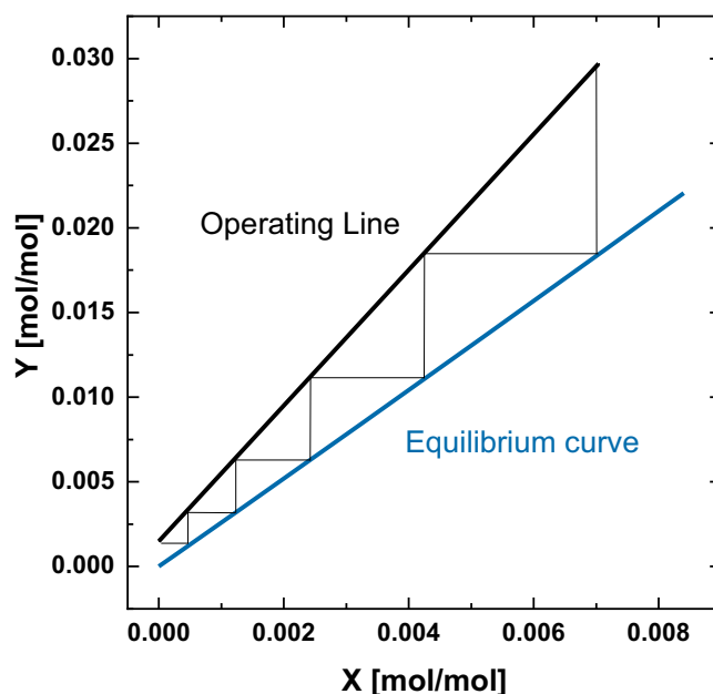
Fig. 10 Design of absorption column. Construction of operating line and equilibrium curve for the determination of the number of necessary theoretical separation stages for the recovery of acetaldehyde from the gaseous stream via absorption in water.
