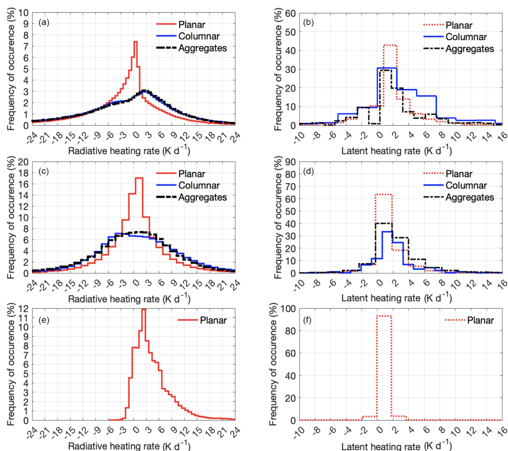
Figure 19. Histograms of diabatic heating in the TTL from microphysics ( b , d , f ) and radiation ( a , c , e ) in the deep-convection ( a , b ), thick-anvil ( c , d ), and thin-cirrus ( e , f ) regions for different ice habits, i.e., columnar (blue) planar (red), and aggregate (black).
