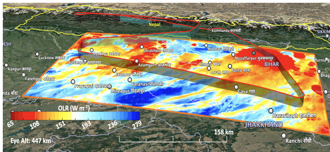
Figure 5. High-resolution (0.3 km) simulated OLR at 10:00 UTC on 10 August 2017. The map was made using © Google Earth 2022.
