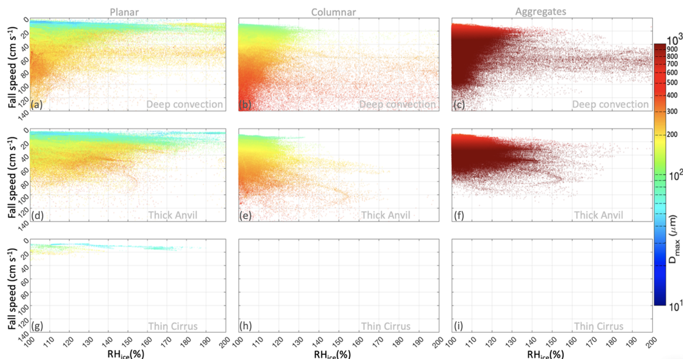
Figure 16. Scatter plots of ice particle fall speed as a function of relative humidity with respect to ice (RH i ), color coded by maximum dimension ( D_{\max} ) for three different ice habits, i.e., planar (a, d, g), columnar (b, e, h), and aggregate (c, f, i), and three different regions, i.e., deep convection (a–c), thick anvil (d–f), and thin cirrus (g–i).
