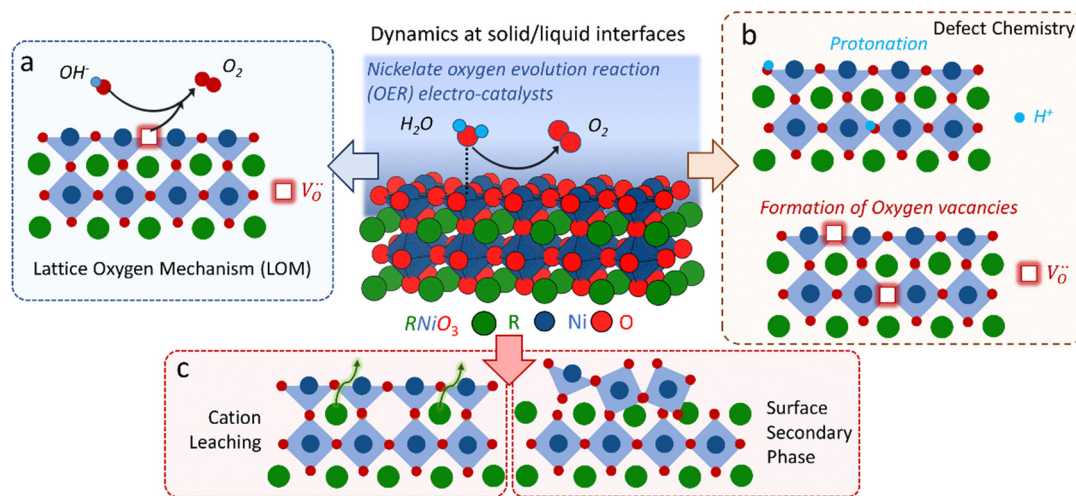
Fig. 1 Dynamic changes of nickelate OER electrocatalysts with the perovskite crystal structure. (a) Lattice oxygen mechanism; (b) formation of ionic point defects; (c) surface compositional change and formation of secondary phases.
