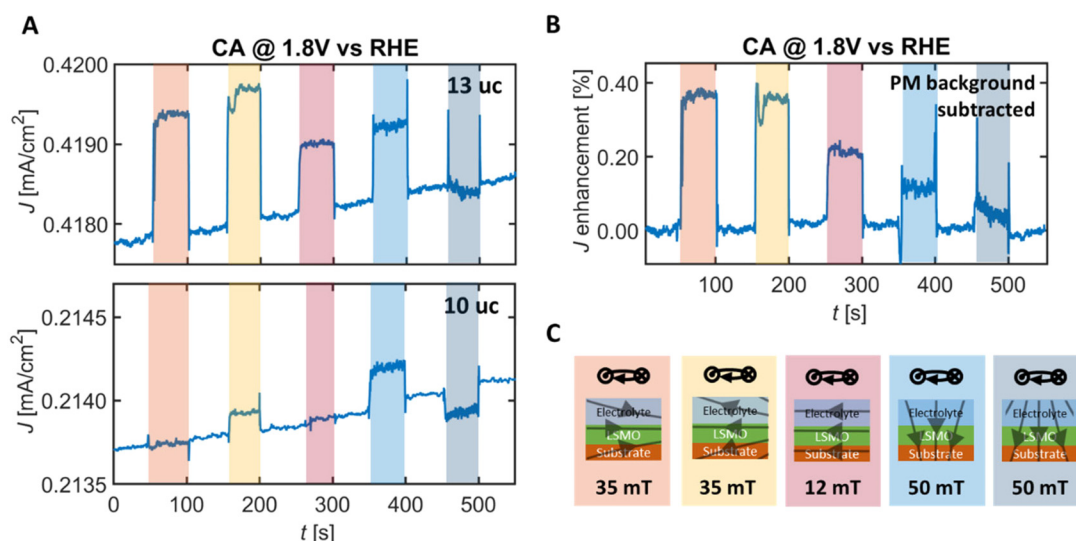
FIG. 6. (a) Chronoamperometry measurement at an potential of 1.8 V vs RHE for a 13 uc and a 10 uc thick \text{La}_{0.67}\text{Sr}_{0.33}\text{MnO}_3 film during which an external magnetic field was applied in different directions. The colored bars indicate the intervals during which the field was applied. The color of the bar represents the direction of the field and corresponds to the colors indicated in Fig. 4. (b) Normalized current density enhancement due to ferromagnetic interactions after paramagnetic background subtraction. (c) Schematic drawing of the field lines in the samples and in the electrolyte. The arrow on top indicates stirring direction.
