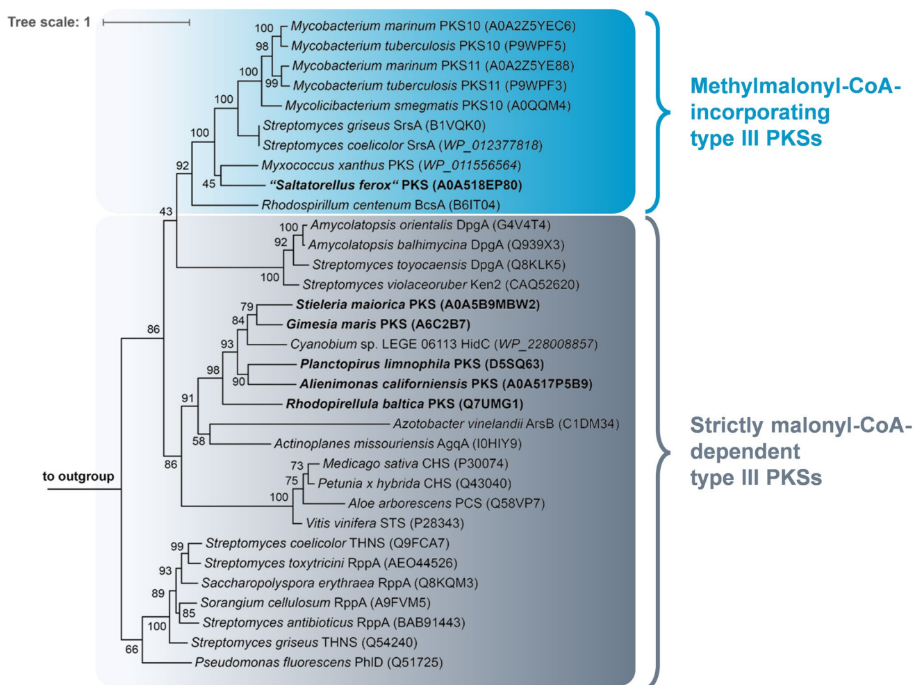
Fig. 5 Phylogenetic tree of the investigated planctomycetal type III PKS and enzymes of this class with an identified reaction product from other organisms. The tree was constructed based on an alignment of type III PKS protein sequences. The sequences of citrate synthase of C. glutamicum (Uniprot-ID P42457) and FtsZ of E. coli
