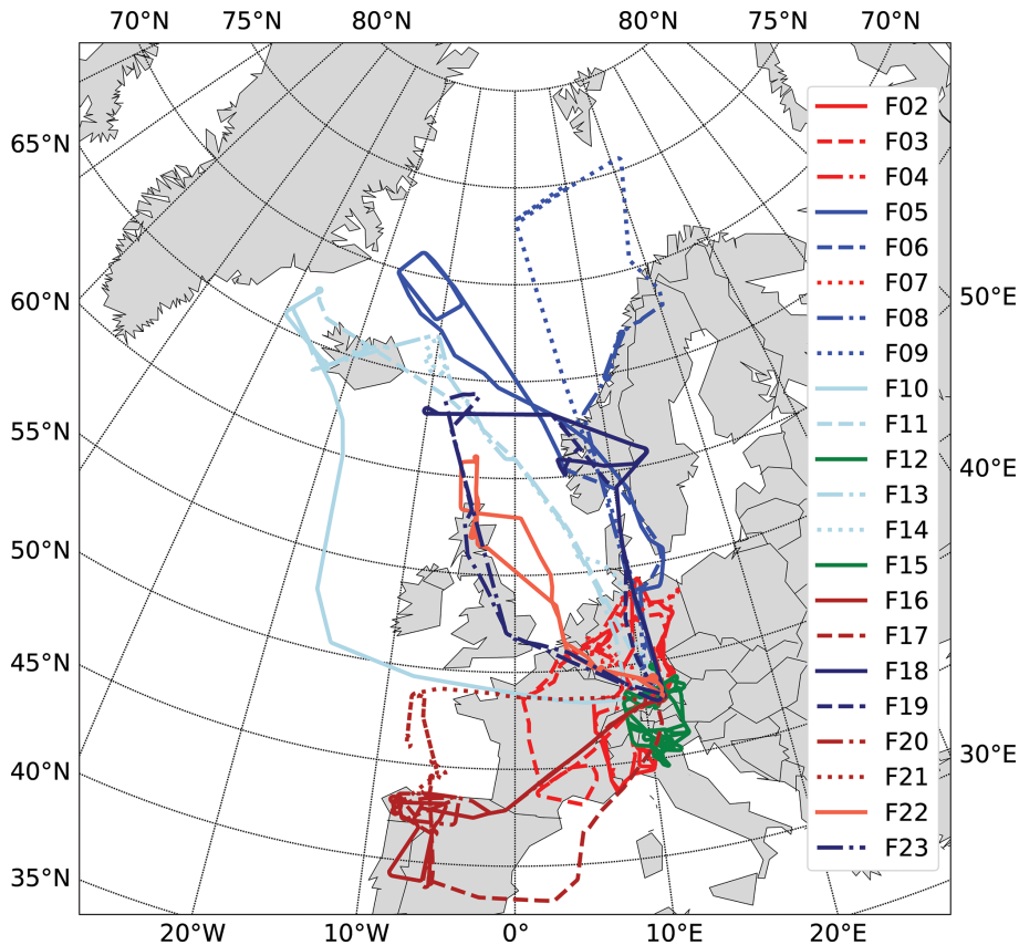
Figure 1. Map of the study region in the Arctic, North Atlantic, and central Europe during the CIRRUS-HL mission in 2021. Each flight is labelled and drawn in a different colour and line style. Flights at high latitudes are indicated with blue colours, red colours represent flights at mid-latitudes, and green is applied for flights in convection.
