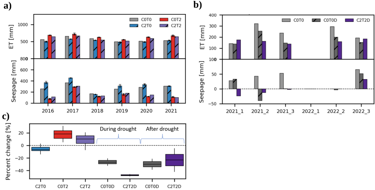
Figure 2. Major components of the water budget from lysimeters from the six core climate manipulation treatments spanning the 2016-2022 growing seasons. Large weighable lysimeter (COT0: n = 1 ; C2T0: n = 2 ; COT2: n = 2 ; and C2T2: n = 1 ) information is displayed in a) , SmartField Lysimeter (SFL) information (COT0: n = 1 ; C2T0: n = 2 ; COT2: n = 2 ; and C2T2: n = 1 ) on a per-cut basis in b) , and c) shows percent deviation from COT0 evapotranspiration (ET) for the years 2016-2022 via combining records from large lysimeter and SFL's. See Figure 1 for treatment code description.
