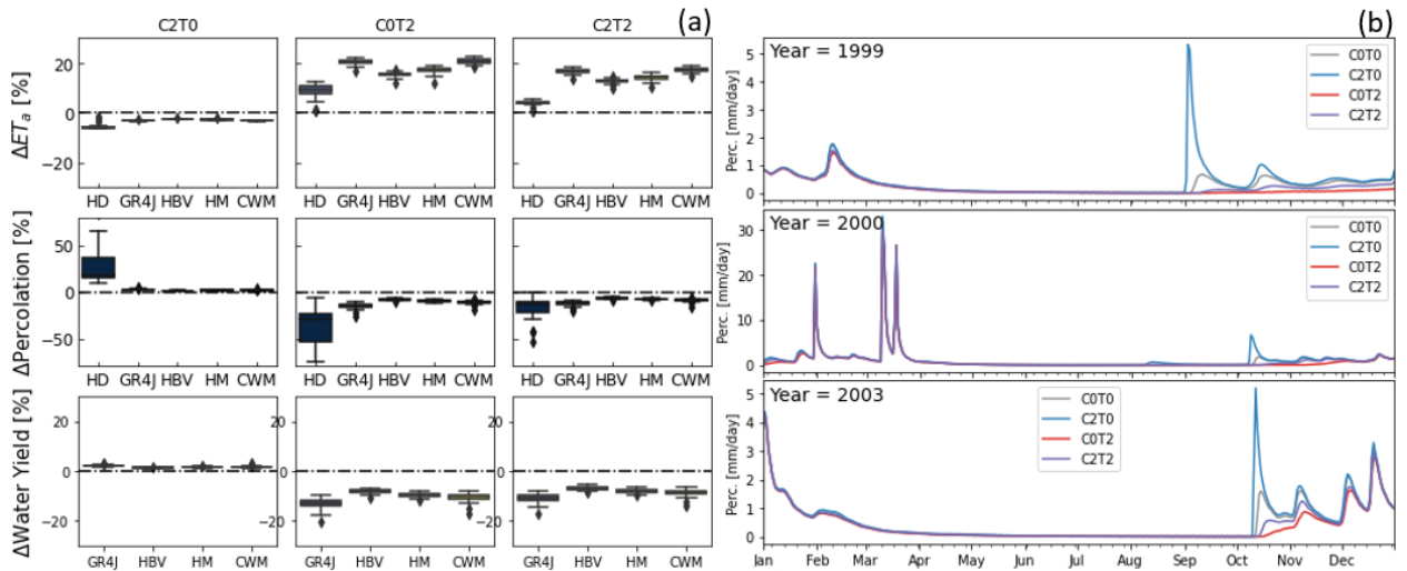
Figure 17: a) Modeled actual evapotranspiration (ETa), percolation, and water yield responses to elevated CO 2 , warming, and their combination compared to ambient conditions for HYDRUS-1D (HD), GR4J, HBV, HYMOD (HM), and CWatM (CWM). b) The hydrological response to different climate treatments is enhanced after dry summer periods at the plot level (HYDRUS-1D). See Figure 2 for treatment code description.
