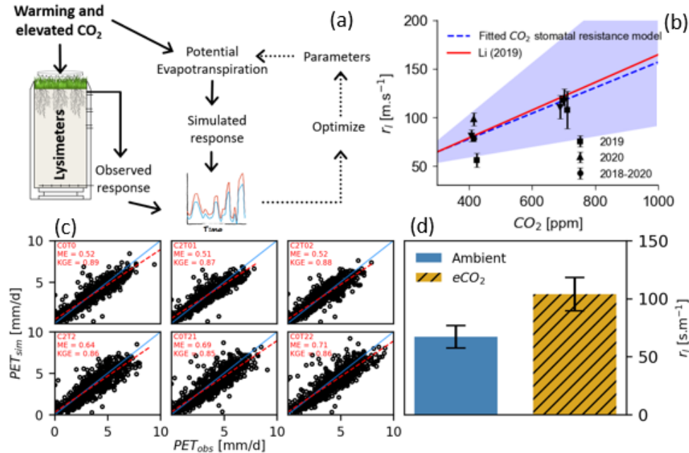
Figure 14. a) Schematic representation of the workflow to estimate the sensitivity of stomatal resistance to elevated \text{CO}_2 concentration. b) Fitted relationship between stomatal resistance ( r_l ) and \text{CO}_2 . c) Comparison between simulated PET and observed PET at the lysimeters. d) Estimated stomatal resistance for ambient conditions and elevated \text{CO}_2 conditions (+300 ppm \text{CO}_2 ) (Adapted after Vremec et al. 38 ).
