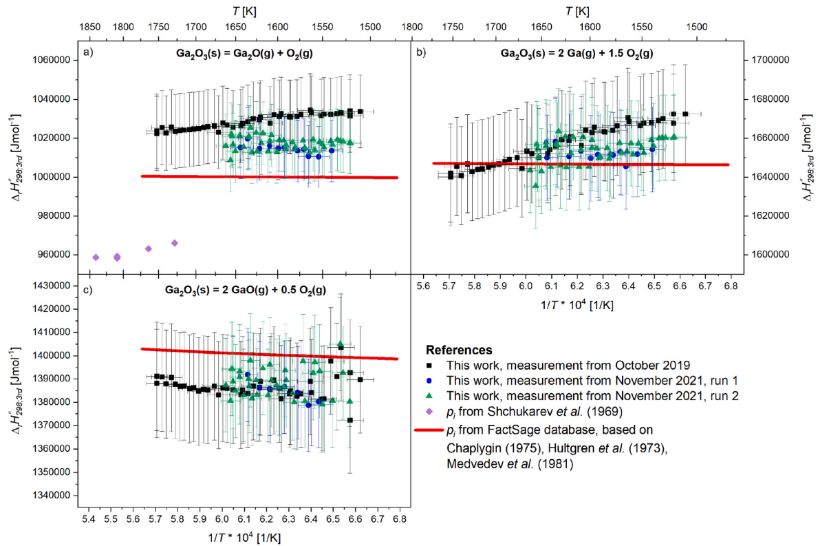
Fig. 9. \Delta_r H^\circ_{298,3rd} for the reactions of \text{Ga}_2\text{O}_3 into a) \text{Ga}_2\text{O} , b) \text{Ga} and c) \text{GaO} plotted vs. reciprocal T for measured and literature data.
