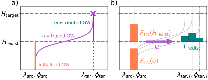
Figure 5.2: Schematic of the construction of transport matrices and the according redistribution of GWMF. Panel a) shows the basic idea of the construction of the transport matrix. For each MWM-initialized MW (violet line), the source and target locations, (\phi_{\text{src}}, \lambda_{\text{src}}) and (\phi_{\text{tar}}, \lambda_{\text{tar}}) , are estimated. The target location is estimated at a set target height, H_{\text{tar}} , and the corresponding amplitude at that altitude serves as the weight for the transport matrix. Once implemented in a parameterization scheme, the propagation is approximated by vertical propagation at the source location up to the redistribution height H_{\text{redist}} (orange line) and at the estimated target location of the original ray-traced MW beyond (teal line). Repeating this process for every launched MW gives the total transport matrix. Panel b) shows a schematic of the full redistribution process as implemented by Eichinger et al. (2023). Following the upward propagation of the total column GWMF in any given grid column up to the redistribution height (orange bars), the total GWMF at that altitude, F_{\text{src}}(H_{\text{redist}}) , is redistributed to multiple grid cells according to the transport matrix \mu to get the redistributed GWMF distribution F_{\text{redist}} (teal bars).
