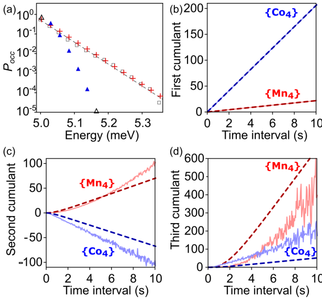
FIG. 7. (a) Occupation probability of the different levels found in the \{Mn_4\} -device on a logarithmic scale for the direct current data (black squares) and for models assuming 50 independent two-level fluctuators (blue triangles) and 50 coherently coupled two-level fluctuators (red crosses). The dashed line is a fit of the data to an exponential distribution. (b) First factorial cumulant ( C_{F,1} ) as extracted from the measurements on the carbon nanotube (CNT) quantum dots functionalized with \{Mn_4\} (red) and \{Co_4\} (blue) complexes. Fits (dashed lines) yield the transition rates used for modeling, in (c), the second ( C_{F,2} ) and, in (d), the third ( C_{F,3} ) factorial cumulant. The solid lines in (b)–(d) are the respective cumulants extracted directly from the digitized measurement signal of the two devices ( \{Mn_4\} : red, \{Co_4\} : blue). The positive second cumulant in (c) is related to a super-Poissonian Fano factor by F = (C_{F,2}/C_{F,1}) + 1 . All lines of the \{Co_4\} sample are multiplied by a factor of 20 for better visibility.
