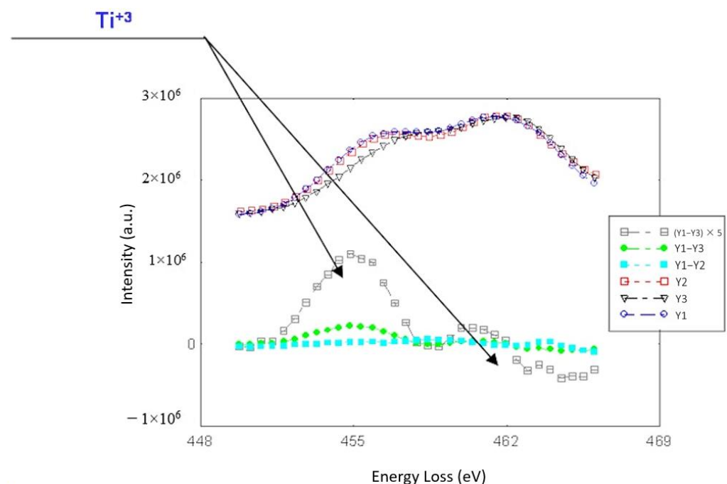
Figure 5. A set of three EELS spectra of the Ti L2,3 line measured for position marked in Figure 4. The relative difference between the spectra (related to the existence of Ti with valence of 3+) is shown at the bottom of the graphs for LSTO-5%La.
