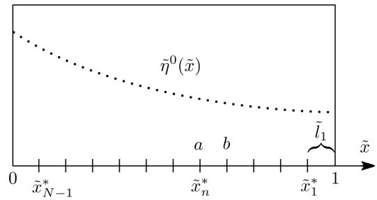
Figure 1. The scheme of the catalyst layer division into N sub-layers. The function \tilde{\eta}^0(\tilde{x}) is approximated by the stepwise function, which is constant in each sub-layer (not shown).
