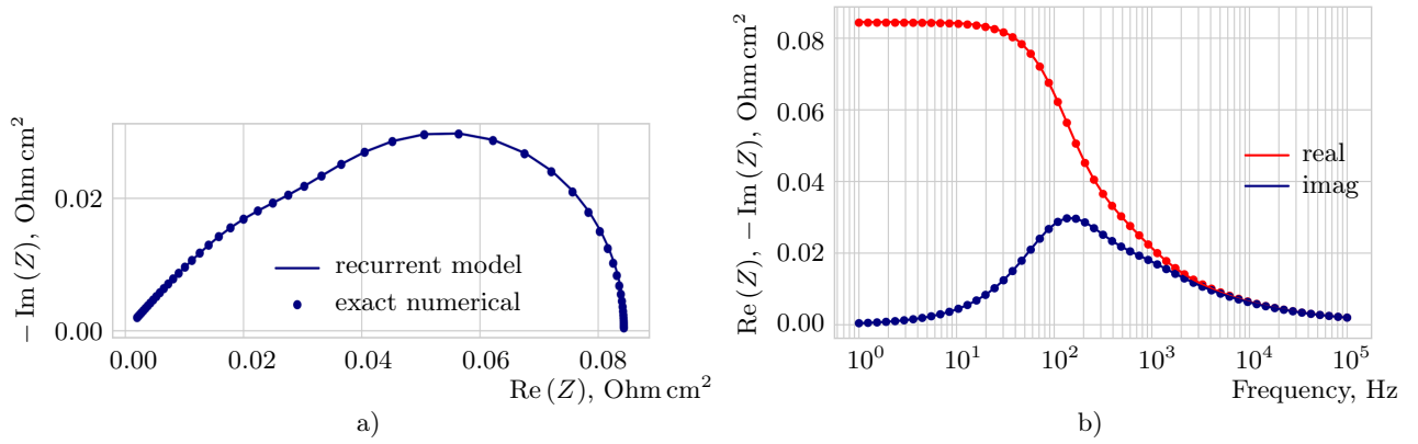
Figure 2. (a) Solid line – the CCL impedance calculated with 10 sub-layers in accordance with the recurrence relation Eq.(11). Points – the CCL impedance computed with help of Eq.(8) and by the direct numerical integration of Eq.(1). In both cases, the static shape of \tilde{\eta}^0 is evaluated from Eq.(6). (b) Real and imaginary parts of the impedance from (a) as a function of frequency \omega .
