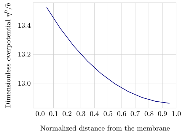
Figure 3. The shape of the dimensionless static ORR overpotential through the CCL depth. The membrane is located at \tilde{x} = 0 .
