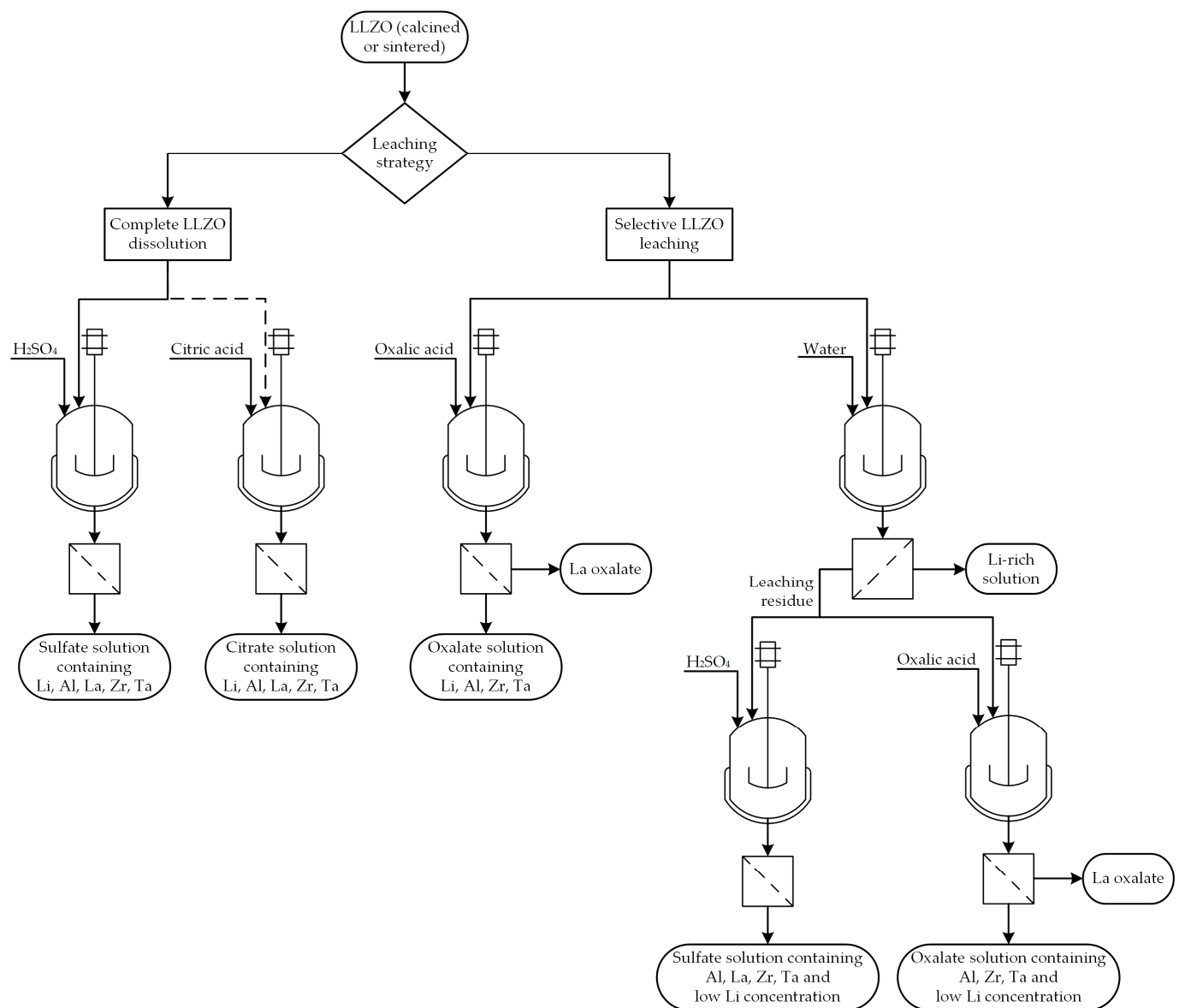
Figure 8. Process approaches for LLZO leaching based on the results of this study. Leaching with citric acid is shown with a dashed line, as the process parameters will need to be optimized for complete dissolution of LLZO.
