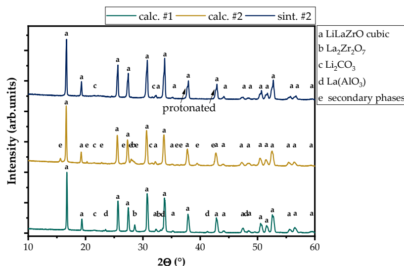
Figure 4. XRD patterns of leaching residues after 24 h leaching in water for calcined LLZO #1, calcined LLZO #2, and sintered LLZO #2. The present phases are cubic LLZO (ICSD: 182312), \text{La}_2\text{Zr}_2\text{O}_7 (ICSD: 015165), \text{Li}_2\text{CO}_3 (ICSD: 066941), and \text{La}(\text{AlO}_3) (ICSD: 090538).
