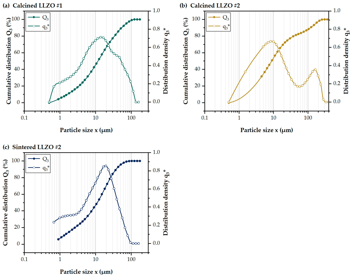
Figure 2. The particle size distribution of the LLZO samples used in the leaching experiments as determined by laser diffraction: calcined LLZO #1 (a), calcined LLZO #2 (b), and sintered LLZO #2 (c).
