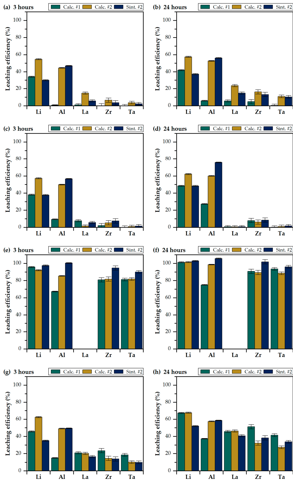
Figure 6. Leaching efficiencies of the calcined and sintered LLZO samples with organic acids: acetic acid (a,b), formic acid (c,d), oxalic acid (e,f), and citric acid (g,h) (acid concentration = 1 M, S:L ratio = 50 g/L, and T = 25 °C). The largest deviation in leaching efficiency was observed for Al, which could be due to an inhomogeneous Al distribution within the samples (see Section 3.2).
