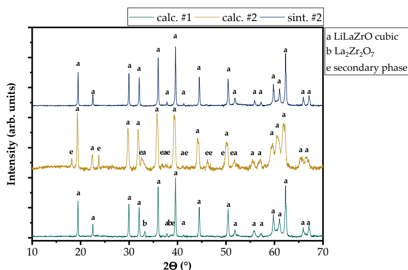
Figure 1. X-ray diffraction (XRD) patterns of calcined LLZO #1, calcined LLZO #2, and sintered LLZO #2. The present phases are cubic LLZO (ICSD: 182312) and \text{La}_2\text{Zr}_2\text{O}_7 (ICSD: 015165).
