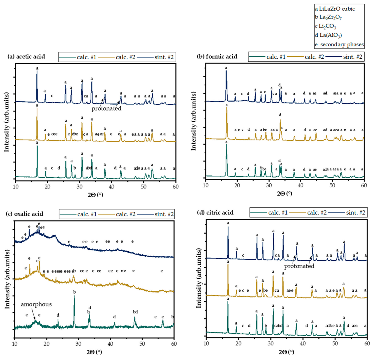
Figure 7. XRD patterns of leaching residues after 24 h of the calcined and sintered LLZO samples with organic acids: acetic acid (a), formic acid (b), oxalic acid (c), and citric acid (d). the present phases are cubic LLZO (ICSD: 182312), \text{La}_2\text{Zr}_2\text{O}_7 (ICSD: 015165), \text{Li}_2\text{CO}_3 (ICSD: 066941), and \text{La}(\text{AlO}_3) (ICSD: 090538).
