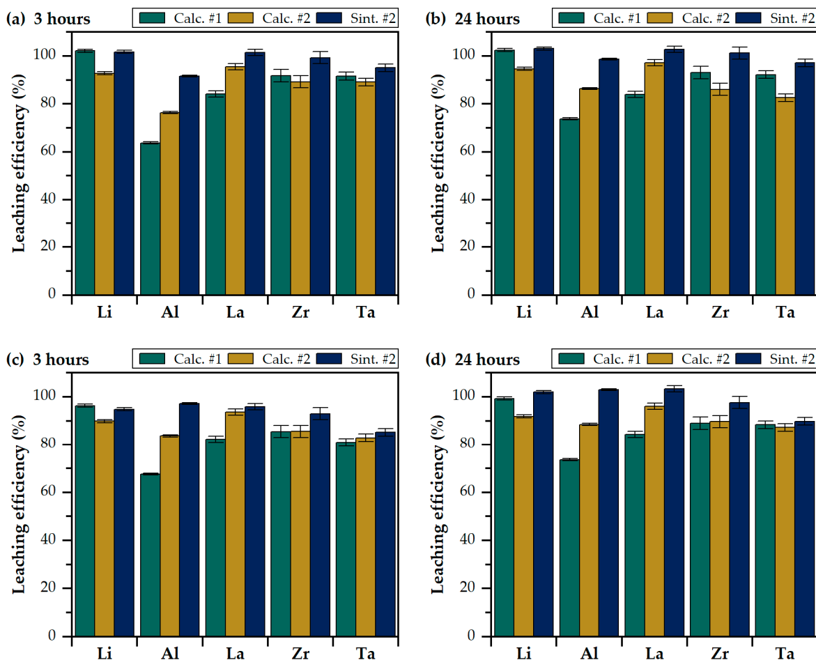
Figure 5. Leaching efficiencies of the calcined and sintered LLZO samples in sulfuric acid after 3 h (a) and 24 h (b) and in hydrochloric acid after 3 h (c) and 24 h (d) (acid concentration = 1 M, S:L ratio = 50 g/L, and T = 25 °C).
