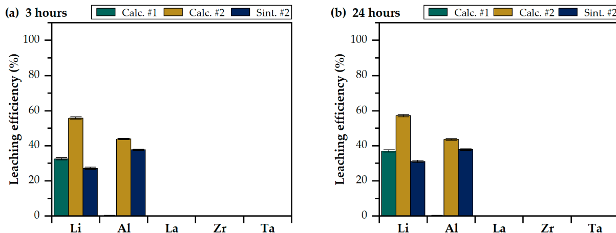
Figure 3. Leaching efficiency of the calcined and sintered LLZO samples in water after 3 h (a) and 24 h (b) (50 g/L of solids and T = 25^\circ ).
