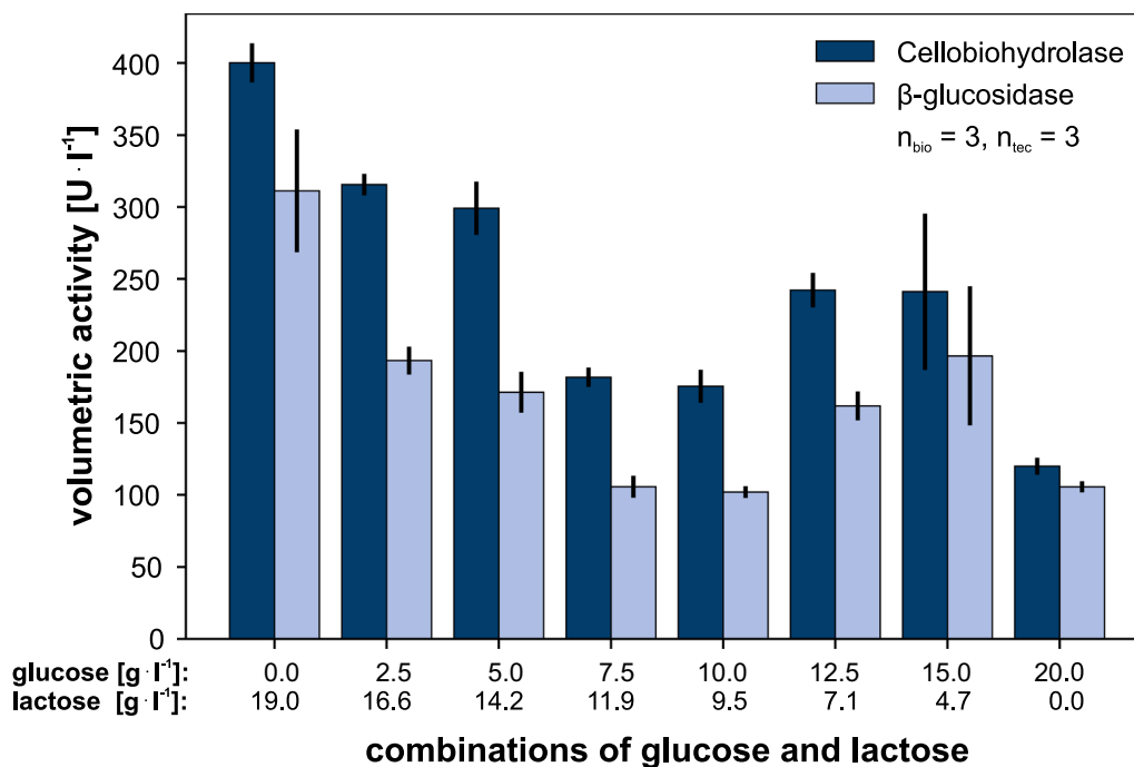
Fig. 5 Volumetric activity of cellobiohydrolase and \beta -glucosidase for different combinations of glucose and lactose. The experiment with 0 g l -1 lactose and 20 g l -1 glucose resulted in the lowest cellobiohydrolase and \beta -glucosidase activities, measuring at 120 \pm 6 U l -1 and 106 \pm 4 U l -1 . The highest cellulase activities of 400 \pm 14 U l -1 and 311 \pm 43 U l -1 were achieved when lactose was used as the sole carbon source. This represents a threefold increase in activity compared to the standard batch approach using glucose as the sole carbon source. Cultivation conditions: RutC30, RWP, adapted medium, n = 1000 rpm, d_0 = 3 mm, V_W = 3.4 ml, V_L = 1 ml, humidity \geq 85\% , O_2 = 35\% , T = 30 °C, inoculum = 10^5 spores ml -1
