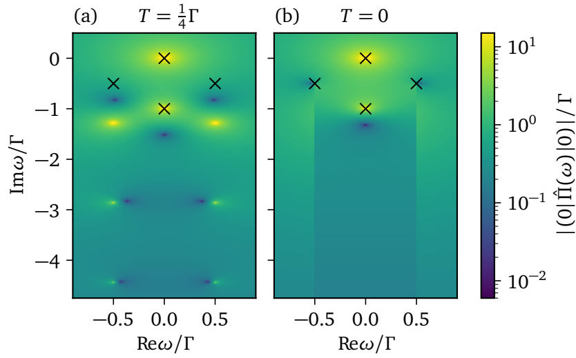
Figure 3: Resonant level model for strong coupling and detuning \varepsilon - \mu = \Gamma/2 . Plotted is the modulus of the complex valued matrix element \langle 0 | \hat{\Pi}(\omega) | 0 \rangle in units of \Gamma in the complex frequency plane where |0\rangle = |0\rangle\langle 0| denotes the unoccupied state. (a) Finite temperature T = \Gamma/4 : distinct from the two infinite sets of equidistant poles there are four poles (marked \times ) at \omega = 0 , \omega = -i\Gamma and \omega = \pm\varepsilon - i\Gamma/2 . The last two poles are not visible here but appear in other matrix elements. (b) For T \rightarrow 0 two branch cuts develop from the sets of equidistant poles. At resonance ( \varepsilon - \mu \ll T ) these poles (branch cuts) cancel exactly leaving just a single pole at -i\Gamma whereas off-resonance ( \varepsilon - \mu \gg T, \Gamma ) they move to the sides where they become suppressed in amplitude. Only in these two limits four poles remain and the dynamics is a semigroup [23]. For T \rightarrow \infty the first case always applies.
