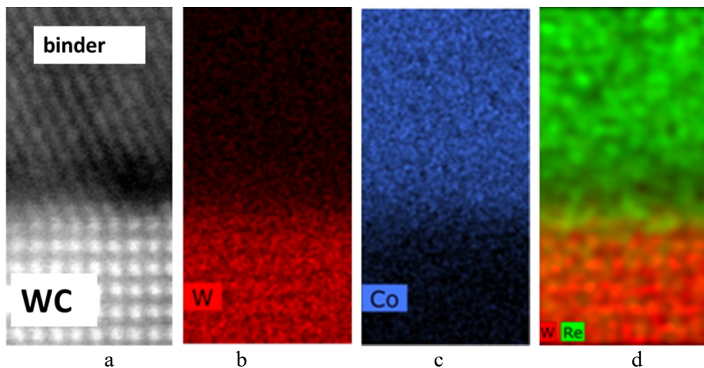
Figure 5. Carbide/binder grain boundary of the WC-Co-Re cemented carbide: a - HAADF STEM image; b and c - corresponding element maps of W and Co; and d – the interface region with red and green spots corresponding to tungsten (red) and rhenium (green) atoms. Note that there is a layer of about 2 to 3 atomic monolayers, in which W and Re atoms are mixed at the WC/binder interface.
