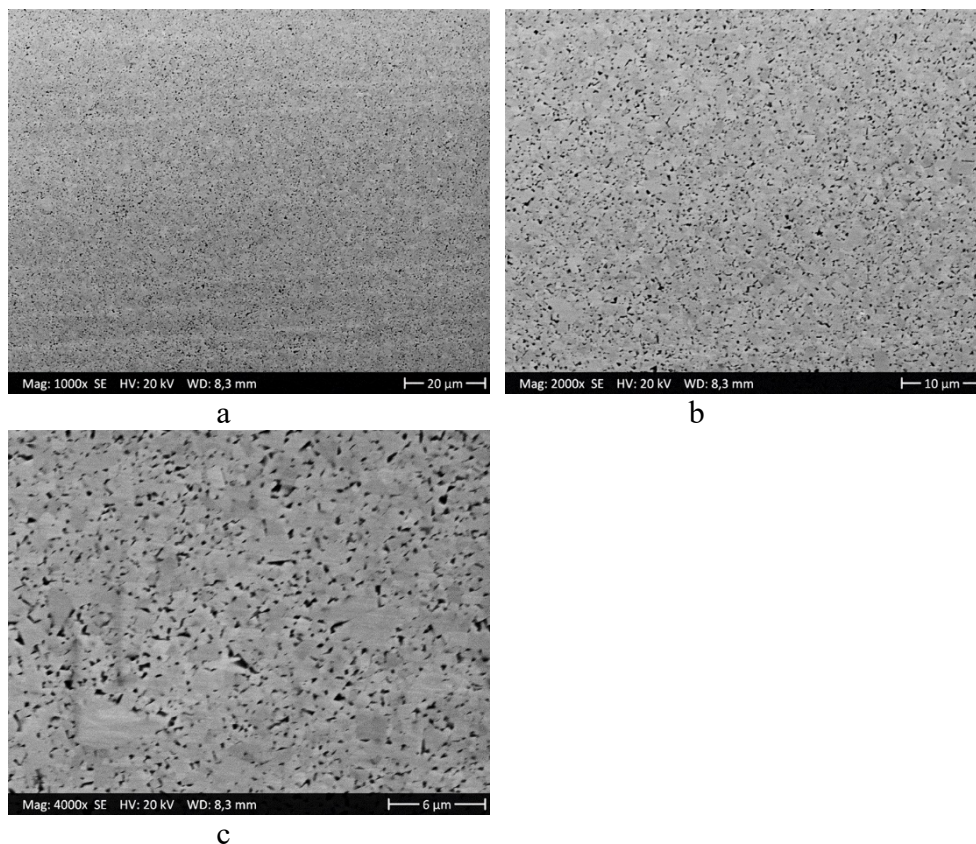
Fig. 1. HRSEM images of the microstructure of the WC-Co-Re cemented carbide at different magnifications: (a) – \times 1000 , (b) – \times 2000 and (c) – \times 4000 .
