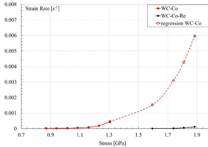
Fig. 3. Curves indicating the dependence of the strain rate on stress obtained when examining the creep process of WC-Co-Re and WC-Co cemented carbides at 800°C after extrapolation of the curve for the WC-Co material.
