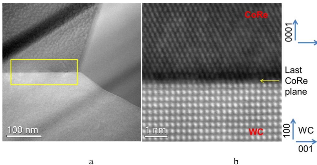
Fig. 4. ADF STEM image of the interfacial region of the WC-Co-Re cemented carbide (a) and HAADF STEM image of the carbide/binder interface (b).
