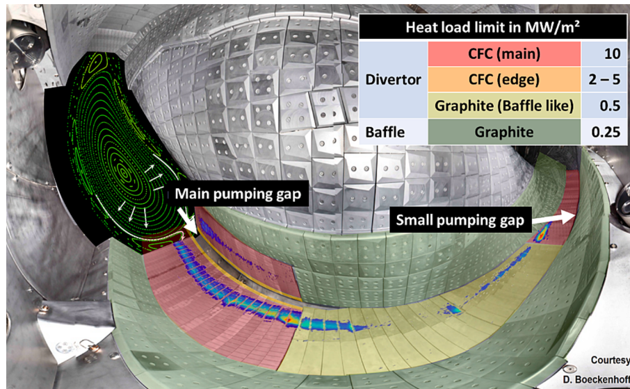
Fig. 2. Plasma facing components with the heat load limits of the CFC divertor and an exemplary overlay of a Poincaré plot of the magnetic field and a heat load pattern.
