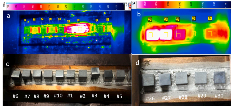
Fig. 4. (a) and (b) IR images showing overheating of samples in batches 1 and 6, respectively. (c) optical images after detachment of #3 (after heat fluxes of < 1 MW/m 2 ) and (d) before the test.
