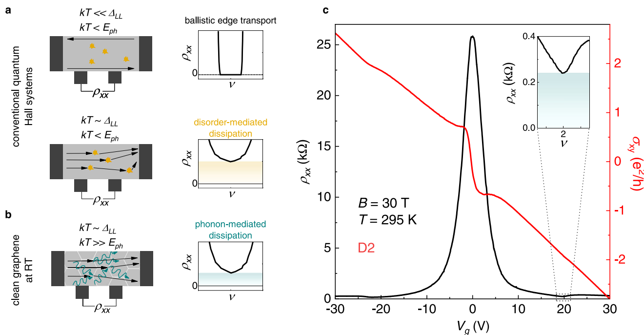
Fig. 1 | Dissipation regimes in the quantum Hall phase: high-quality graphene at RT. a Schematics of temperature-dependent transport in conventional quantum Hall systems, such as 2DEs in semiconductors. At low T (relative to the LL separation, upper part), the electrical current is carried by chiral edge states, leading to zero longitudinal resistance. At higher T (lower part), thermally-excited bulk states give a finite resistivity due to disorder scattering (yellow shading), with negligible contribution from lattice vibrations. b At RT, graphene supports both the
