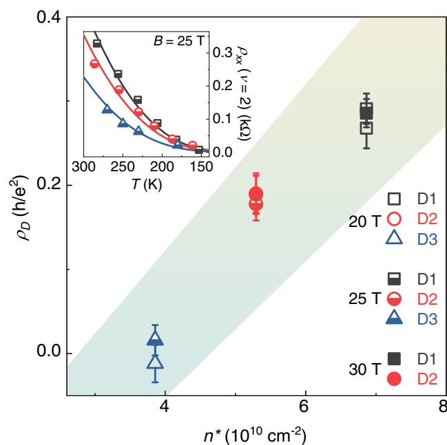
Fig. 4 | Sample-dependent disorder contribution to the activated resistivity. Correlation between the T -independent pre-factor to the activated resistivity and n^* (220 K) for devices D1-3. The shaded area is defined as in Fig. 2b. The error bars correspond to \pm one standard error from the fits shown in the inset. Inset: fits to the minimum resistivity as a function of temperature (continuous lines), using the generalized formula including both e-ph and disorder contributions, at B = 25 T.
