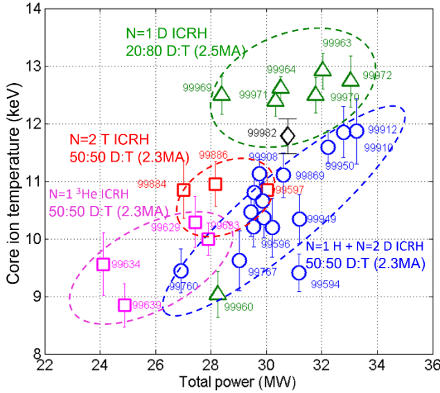
FIGURE 10. Overview of the hybrid-scenario type pulses with different ICRH schemes: Ion temperature (crystal spectroscopy) is plotted vs total heating power, data averaged over 8-9 sec. Pulses with \omega=\omega_{c,H} ICRH are represented with blue circles. The pure \omega=2\omega_{c,T} ICRH pulses are with red squares and the ones using \omega=\omega_{c,3He} ICRH with magenta squares. The tritium-rich plasmas using \omega=\omega_{c,D} ICRH are with green triangles. 99982 is a 3-ion scheme test reported in [34].
