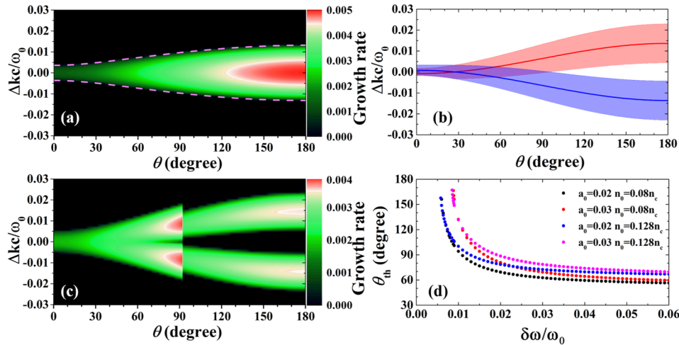
FIG. 1. Linear theory of the SRS growth rate for a two-color laser. (a) Distribution of SRS growth rate \Gamma calculated according to Eq. (1) with a_0 = 0.02 and n_0 = 0.128n_c . Here, \Delta k = \sqrt{(k_x - k_0)^2 + k_y^2} - k_{sr} and \theta = 180^\circ - \arctan[k_y/(k_x - k_0)] . The resonance point k_{sr} is defined by the wave vector and frequency matching conditions of a monochromatic laser beam. (b) Region for \Gamma > 0 as a function of scattering angle ( \theta ) for two individual laser beams at frequencies \omega_0 \pm 0.5\delta\omega , denoted by the red and blue regions, respectively. Here, \delta\omega/\omega_0 = 1.2\% , and a_{1,2} = 0.0141 . The solid red and blue lines are the resonance points calculated using Eq. (3), and the width of each instability region is calculated using Eq. (2). (c) Growth rate as a function of scattering angle calculated using Eq. (5) for two-color laser light with \delta\omega/\omega_0 = 1.2\% . (d) Coupling threshold angle \theta_{th} as a function of the frequency difference \delta\omega between two individual monochromatic laser beams.
