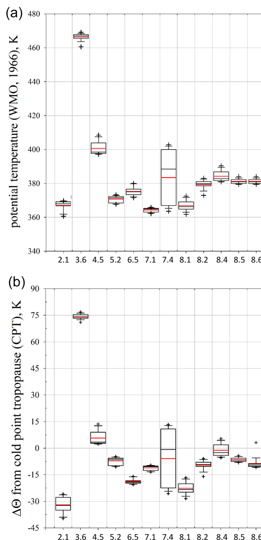
Figure 1. Boxplot of the absolute potential temperature \Theta (a) and of the potential temperature \Theta difference to the 1 Hz calculated \Theta level of the cold point tropopause (CPT) throughout the sampling period (b).
