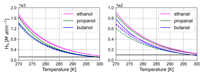
Figure 5. Comparison between estimated and experimental H_s as a function of temperature. Solid lines denote experimental and dashed lines estimated values. The solid black line denotes H_s at 298 K with no further temperature correction. Experimental data are taken from Staudinger and Roberts (2001).
