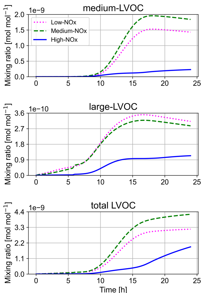
Figure 8. \text{NO}_x dependence of the LVOC formation. Results are displayed for low- \text{NO}_x (dotted magenta line), medium- \text{NO}_x (dashed green line) and high- \text{NO}_x (solid blue line) \text{NO}_x mixing ratios. For definitions of low, medium, and high, see the main text.
