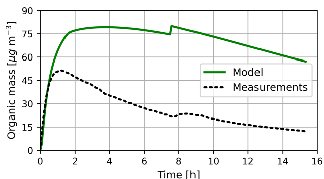
Figure 10. Mass concentration of OMC in the model and experiment. Modelled OMC represents all species with an H_s larger than 4 \times 10^6 \text{ M atm}^{-1} in either the gas phase or the aqueous phase. This simplification is applied to account for missing processes in the model. After 7.5 h, NO is injected into the chamber.
