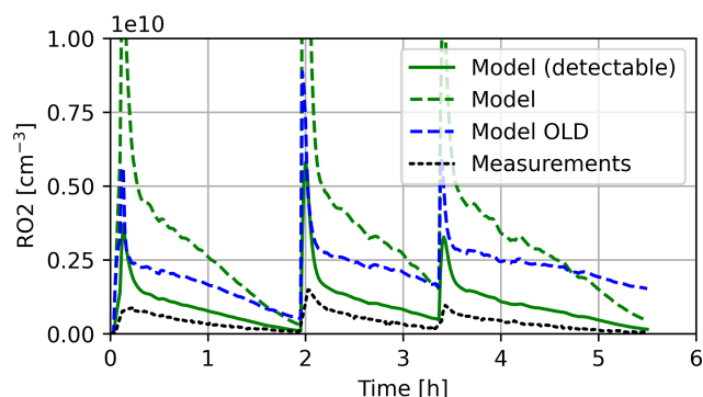
Figure 11. \text{RO}_2 mixing ratios in the model and experiment. Model results marked as detectable are modified by \text{HO}_x formation efficiencies by Vereecken et al. (2021).
