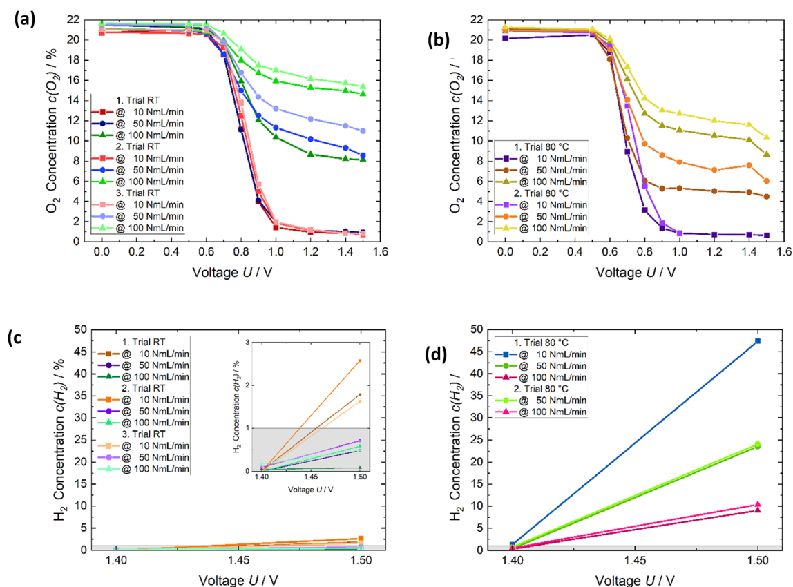
Fig. 6 (a) Measured oxygen content for all trials at room temperature, (b) measured oxygen content for all trials at 80^\circ\text{C} , (c) measured hydrogen content for all trials at room temperature, and (d) measured hydrogen content for all trials at 80^\circ\text{C} .
