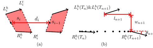
Fig. 1. Spatial structure of walking. (a) Definitions of spatial state( P_i ), head position and physical space ( s_i ). (b) Definition of step width ( w ), step length ( l ) and foot open angle ( \theta ).
