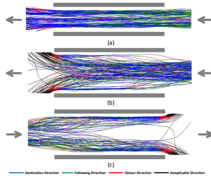
Figure 6. Featured trajectories in uni and bi-directional flow (color). The trajectories are colored with blue, green, red and black to represent destination, following, detour and inexplicable direction, respectively. (a) Pedestrian trajectories of uni-directional flow experiment. (b) Pedestrian trajectories from right to left in bi-directional flow experiment. (c) Pedestrian trajectories from left to right in bi-directional flow experiment.
