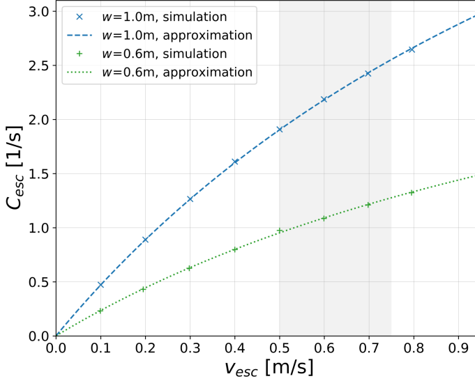
Figure 8. Non-linear speed-dependence of the escalator capacity. Shown are simulation results for the escalator widths w=1.0 m (blue markers) and w=0.6 m (green markers). The respective approximations are obtained by using Eq. (16) with d_{step}=0.4 m and T=0.25 s. The shaded area indicates the range of typical escalator speeds.
