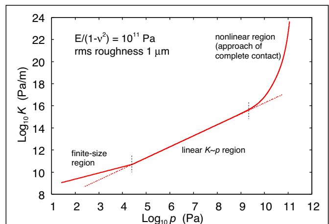
Figure 8. The perpendicular contact stiffness as a function of the squeezing pressure (log-log scale). For an elastic solid with E^* = E/(1 - \nu^2) = 100 GPa and with a randomly rough (self-affine fractal) surface with the rms-roughness amplitude 1 \mu\text{m} .
