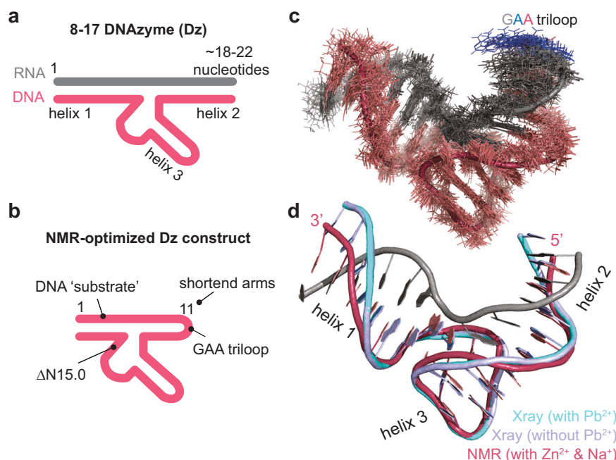
Fig. 1 | Overview of the 8–17 DNzyme (Dz) system. Schematics of the general Dz design (a) and the construct designed for NMR studies (b). c NMR ensemble (20 structures) determined by Wieruszecka, Pwlowicz et al. 5 using the construct shown in (b). For simplicity the substrate sequence of the all-DNA construct is shown in grey and the GAA-triloop in indicated colours. d Comparison of
