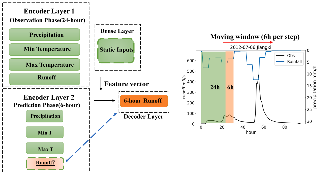
Fig. 3. Input composition and prediction process of the ED-LSTM structure for one event. Two encoder layers incorporated previous 24-hour data in the observation phase and 6-hour pseudo forecasting meteorological data as driving forces (all of these data were observations). The decoder layer outputs the predicted 6-hour runoff corresponding to a 6-hour driving force in the prediction phase. The dense layer functions as an embedding layer for feeding the catchment static variables. For one event, the two phases consist of a moving window and each step moves them forward in 6-hour increments.
