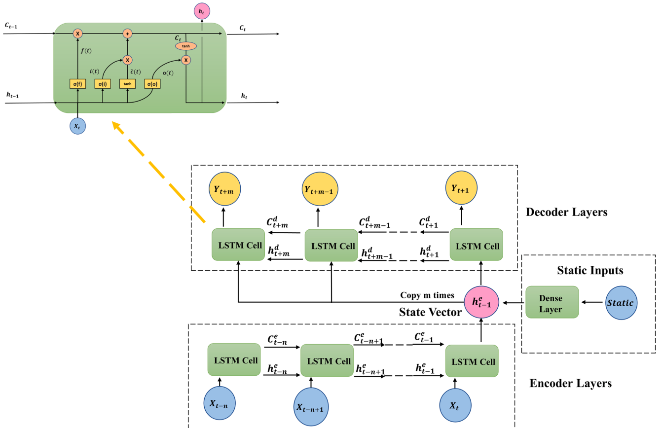
Fig. 2. Configuration of the LSTM cell: \sigma and \tanh represent sigmoid and tanh activation functions, respectively. x represents the input while c and h are the cell state and hidden state at the current time step.
