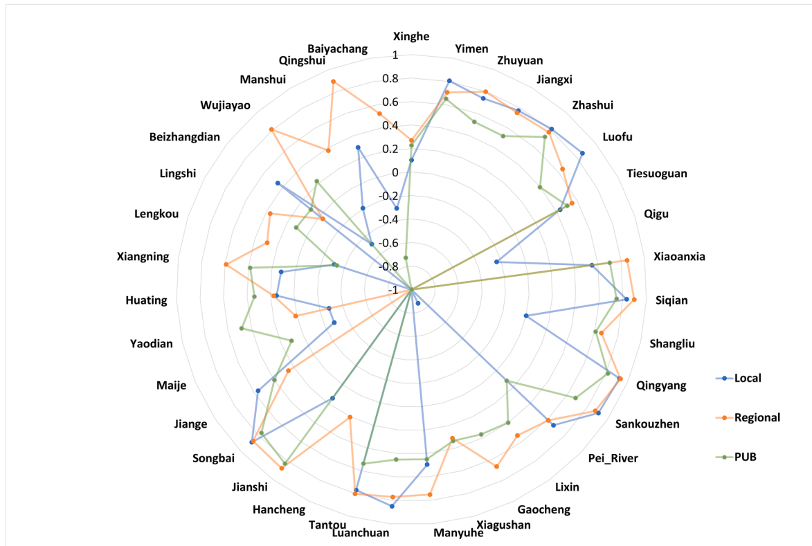
Fig. 6. Radar plot for showing median NSE at 35 catchments for all events of local, regional, and PUB experiments.
