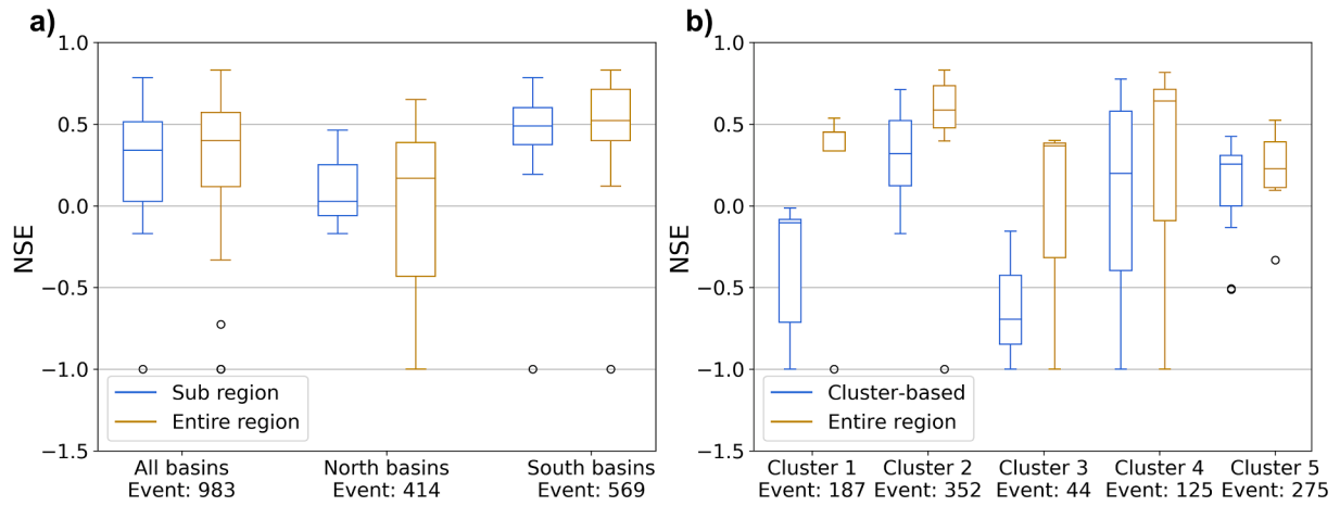
Fig. 5. Boxplot of NSE for PUB models, comparing the models trained on sub-regional areas: (a) north and south regions; (b) hydroclimatic clusters. The line inside the box shows the median and the box includes the lower and upper quartile values (the 25th-75th percentile range). The circles represent the outliers. The number of flood events (samples) that are valid for modeling training for each sub-region is listed below each label. For better visualization, NSE values lower than -1 are set to be -1 .
