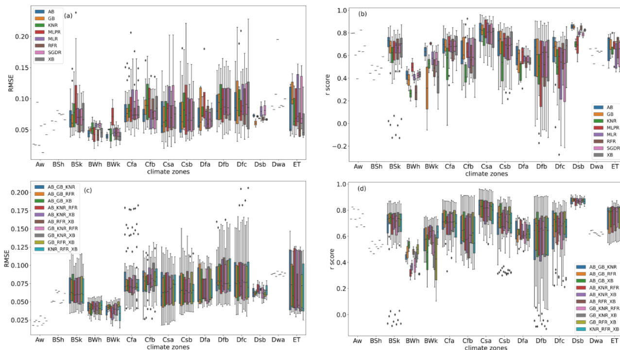
Figure 4. Box plot of the RMSE and r score for the test_independent-stations set based on climate zones: the performance of 8 optimised ML algorithms can be found in panels (a) and (b), while the performance of 10 ensemble models are shown in panels (c) and (d). The abbreviations used in the figure for the climate zones are as follows: Aw – tropical wet and dry or savanna climate, BSh – hot semi-arid climate, BSk – cold semi-arid climate, BWh – hot desert climate, BWk – cold desert climate, Cfa – humid subtropical climate, Cfb – temperate oceanic climate, Csa – hot-summer Mediterranean climate, Csb – warm-summer Mediterranean climate, Dfa – hot-summer humid continental climate, Dfb – warm-summer humid continental climate, Dfc – subarctic climate, Dsb – Mediterranean-influenced warm-summer humid continental climate, Dwa – monsoon-influenced hot-summer humid continental climate, and ET – tundra climate. The abbreviations used in the figure for the ML algorithms are as follows: RFR – Random Forest Regressor, KNR – K-neighbours Regressor, AB – AdaBoost, SGDR – Stochastic Gradient Descent Regressor, MLR – Multiple Linear Regressor, MLPR – Multi-layer Perceptron Regressor, XB – Extreme Gradient Boosting, and GB – GradientBoosting. Note that GB_KNR_RFR refers to the ensemble model constructed by GB, KNR, and RFR, whereas AB_RFR_XB refers to the ensemble model constructed by AB, RFR, and XB. The same naming procedure applies for GB_KNR_XB, GB_RFR_XB, KNR_RFR_XB, AB_GB_KNR, AB_GB_RFR, AB_GB_XB, AB_KNR_RFR, and AB_KNR_XB.
