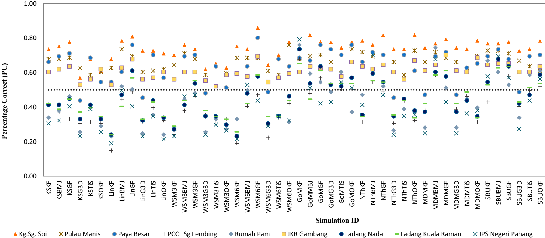
Figure 4. Percentage correct for the WRF physical schemes combination at each station of KRB.
