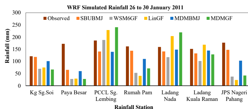
Figure 12. WRF simulated rainfall for the 26 to 30 January 2011 event.
