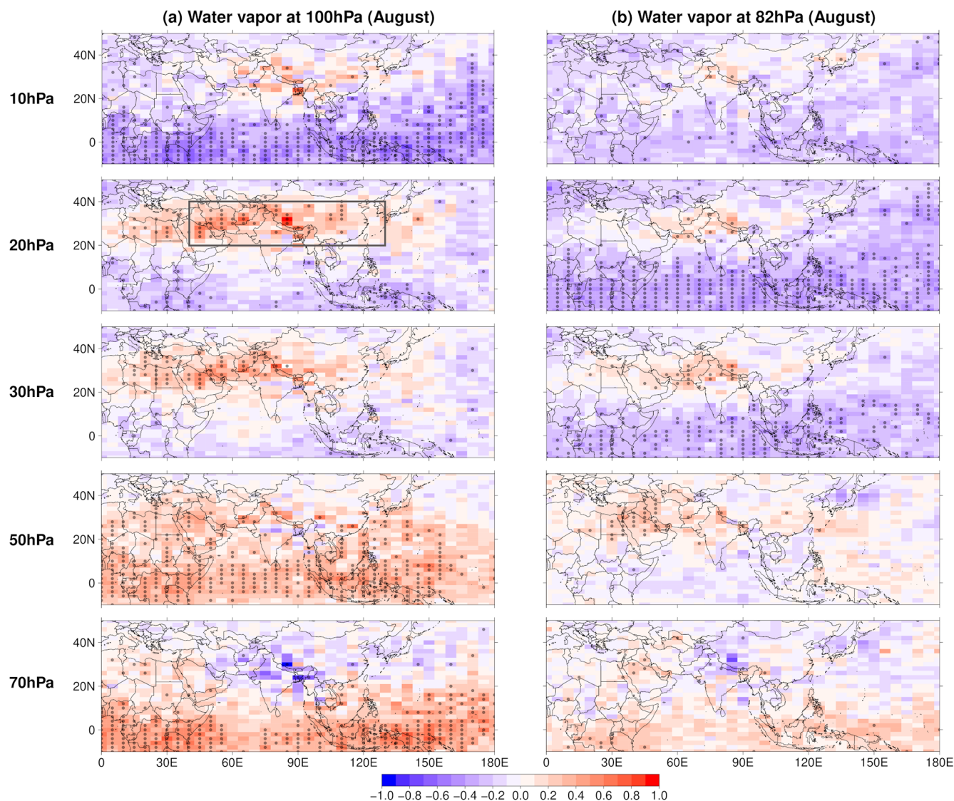
Figure A2. QBO-W minus QBO-E differences for MLS water vapour at 100 hPa (a) and 82 hPa (b) for August over the period 2005–2020. Each row corresponds to a different level at which the QBO phases were defined from 10 hPa (top row panels) to 70 hPa (bottom row panels). Dots indicate significance at the 95 % confidence level. The region inside the grey box corresponds to the Asian monsoon region during the QBO phase in which we have identified a stronger signal on the water vapour of this area.
