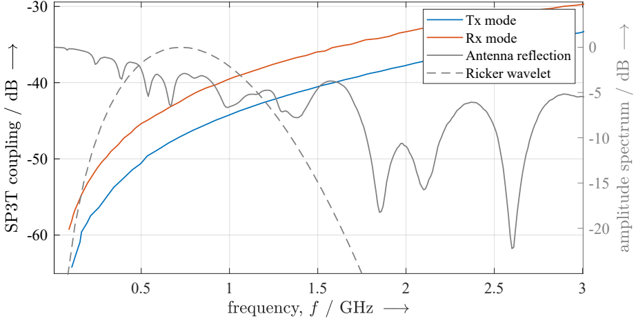
Figure 3.11: Isolation of SP3T switch, scattering parameter of antenna and frequency spectrum of Ricker wavelet.
