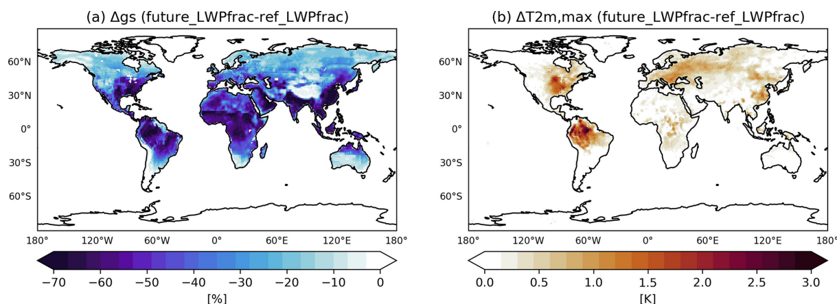
Figure 9. The (boreal) summer mean change in stomatal conductance (a) and daily 2 m maximum temperature (b) when comparing LWPfrac for normal and future conditions (double CO 2 ).
