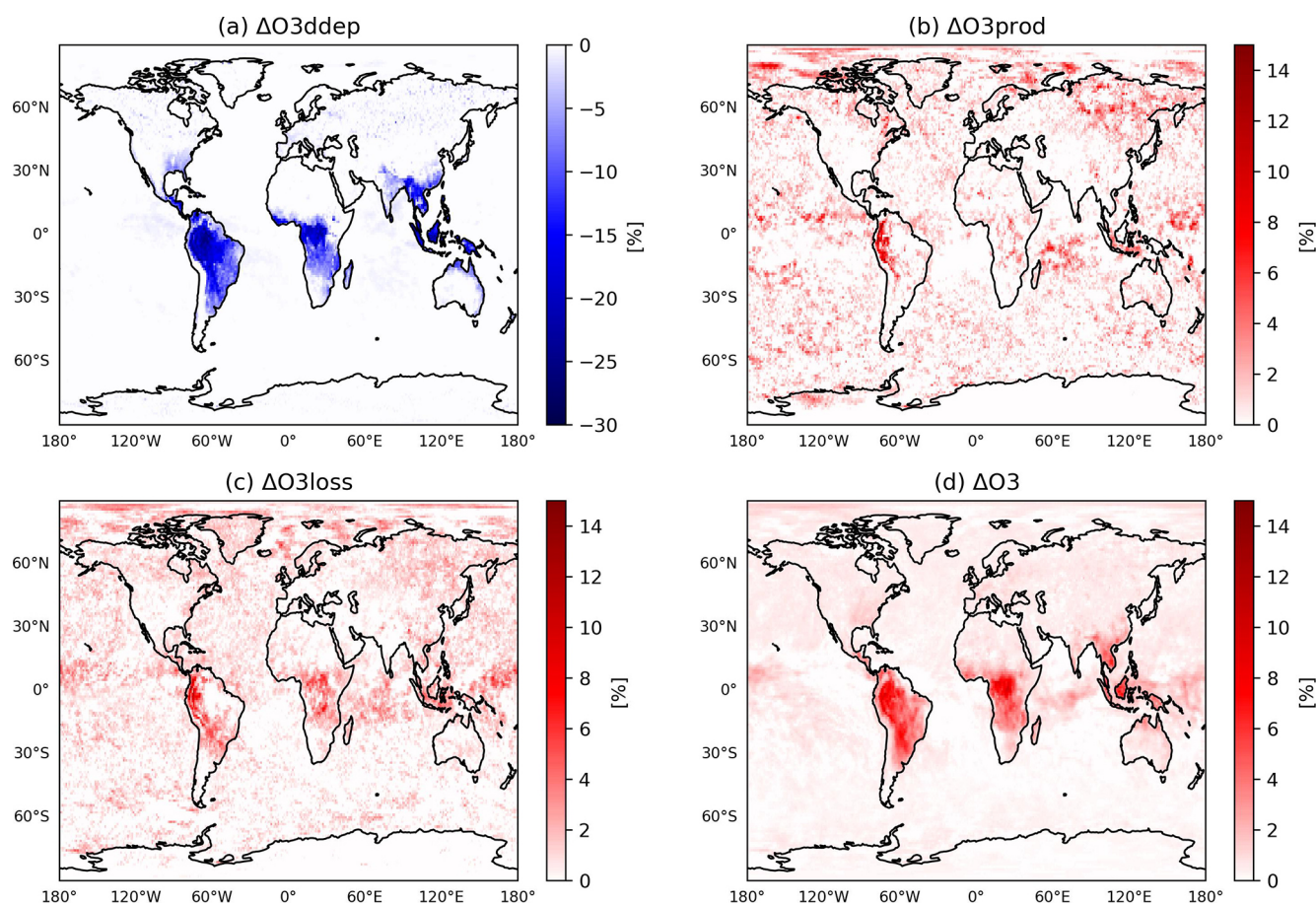
Figure 8. The relative change between LWPfrac and REF of the annual mean (a) O_3 dry deposition, (b) chemical O_3 production, (c) chemical loss, and (d) surface O_3 mixing ratio.
