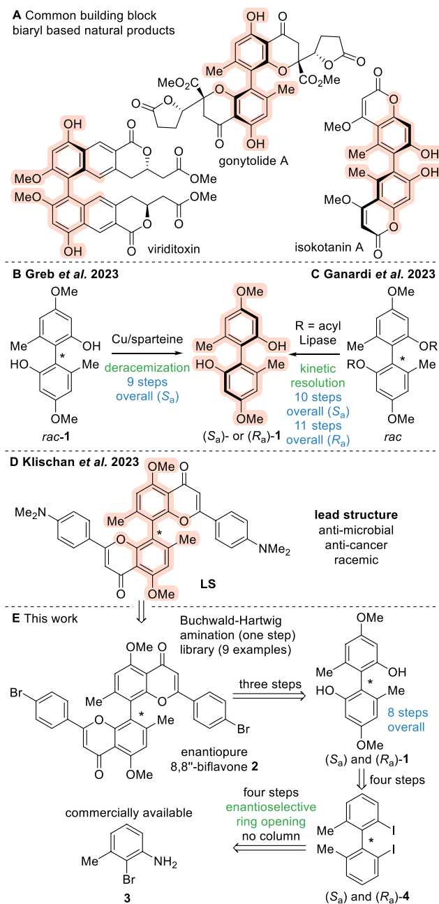
Scheme 1. (A) Biphenol 1 as a Common Building Block in Natural Product Synthesis, (B) Synthesis of Biphenol ( S_a )-1 by Deracemization, (C) Enzymatic Kinetic Resolution of Biphenol 1, (D) Previously Identified Lead Structure (LS), and (E) Enantioselective Synthesis of Biflavones Involving Biphenol Building Block 1
