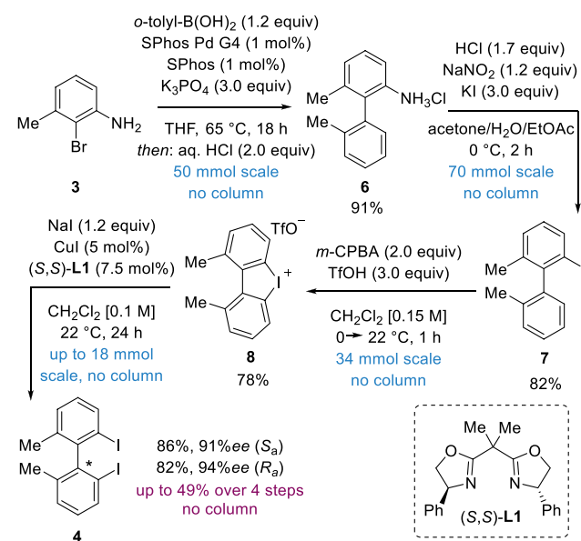
Scheme 2. Synthesis Route toward Both Enantiomers of 2,2'-Diiodo Biaryl 4
