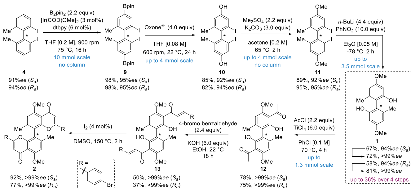
Scheme 3. Synthesis of Biphenol 1 and Its Application in the Synthesis of Both Enantiomers of 8,8''-Biflavone 2
