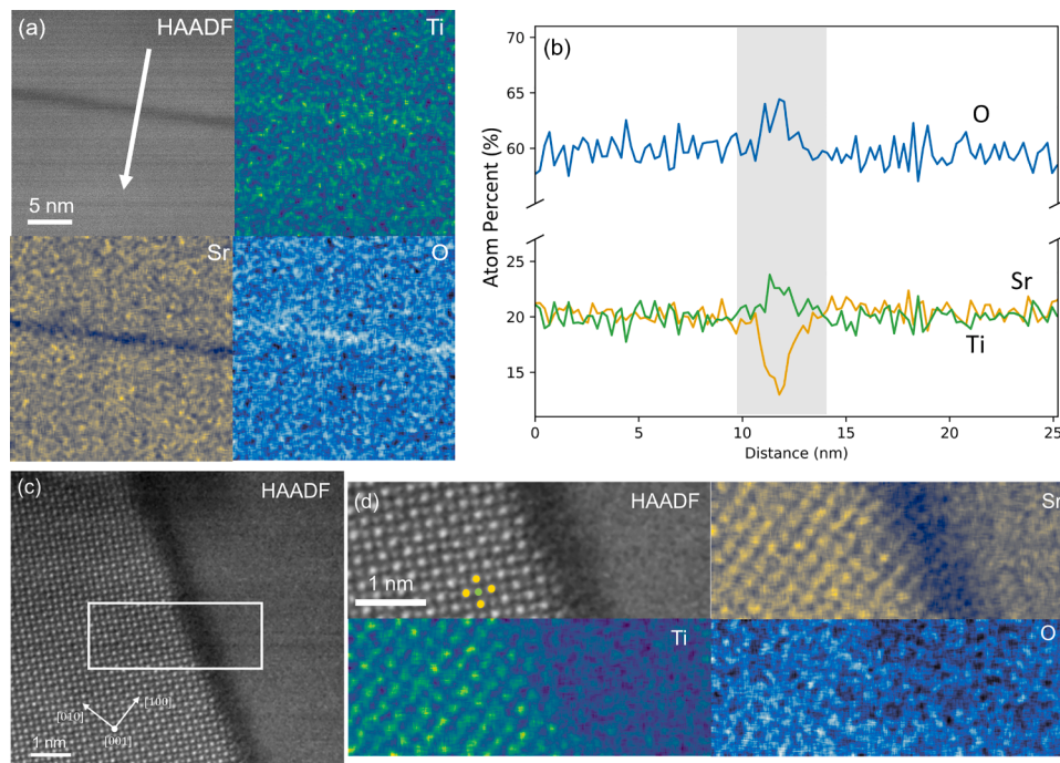
Fig. 2. Low and high-resolution analysis of GB segregation in the undoped sample. (a) EDS mapping of general grain boundary in undoped STO. (b) Line scan of EDS mapping in (a), showing elemental segregation around the grain boundary (gray highlighted region). (c) HRSTEM HAADF image of a general grain boundary in undoped strontium titanate. (d) EDS map of the area within the white box in (c), showing strontium depletion at the grain boundary. One unit cell is overlaid in (d), indicating positions of Sr (yellow) and Ti/O (green) columns. (a) and (b) are reprinted, with permission from Elsevier, from the Journal of the European Ceramic Society, Volume 43: M.P. Zahler, D. Jennings, M. Kindelmann, O. Guillon, and W. Rheinheimer, Reactive FAST/SPS sintering of strontium titanate as a tool for grain boundary engineering , 6925–6933, 2023. [54].
