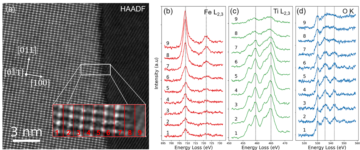
Fig. 7. High resolution EELS analysis of Fe, Ti, and O at a grain boundary of the highly Fe doped (25 % Fe on the B-site) strontium titanate. (a) HRSTEM HAADF image of a grain boundary (the same boundary as Figure S7), and EELS spectra from the nine binned regions in (a) for the Fe L edge (b), the Ti L edge (c), and the O K edge (d).
