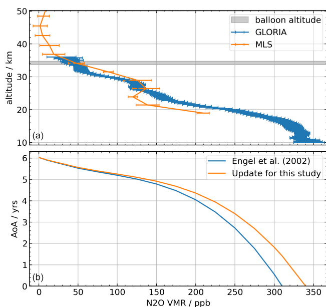
Figure C1. \text{N}_2\text{O} profiles measured by GLORIA and the MLS (a). Panel (b) shows the mean age of air for a given \text{N}_2\text{O} VMR. A measured [\text{N}_2\text{O}] of (40 \pm 20) ppb results in an age of air of around (5.5 \pm 1.0) years since stratospheric entry.
