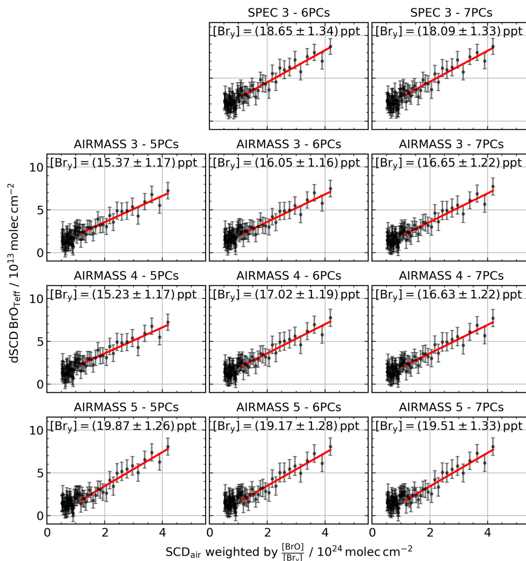
Figure B2. Br y Langley fits for the 11 parameter configurations of the residual correction. The mean [Br y ] is 17.5 ppt. The standard deviation is 1.6 ppt and the mean fit error is 1.2 ppt.
