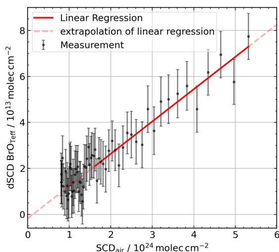
Figure 10. Langley plot for BrO. The dSCD BrO error bars indicate the 1\sigma DOAS retrieval uncertainty. The linear regression (red solid line) yields a slope of [\text{BrO}] = (14.1 \pm 1.0) \text{ ppt} and a y-axis intercept of \text{SCD}_{\text{BrO},0} = (1.8 \pm 3.0) \times 10^{12} \text{ molec. cm}^{-2} . The faint dashed red line indicates the extrapolation of the linear regression outside the fit range of 86^\circ \leq \text{SZA} \leq 89.9^\circ .
