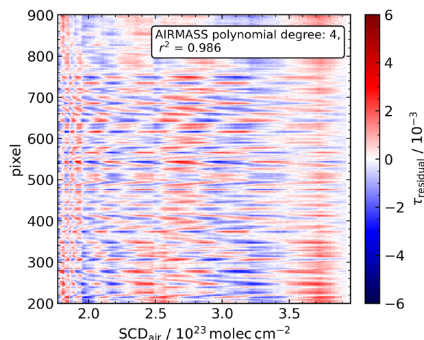
Figure 6. Optical density fluctuations due to residual spectral structures \tau_{\text{residual}} shown for detector pixels 200 to 900 as a function of slant air mass \text{SCD}_{\text{air}} . The spectral pattern was obtained using the AIRMASS approach with a fourth-degree polynomial, as described in the text. The chosen reference spectrum at \text{SZA} = 74.1^\circ has a \text{SCD}_{\text{air}} of 3.9 \times 10^{23} \text{ molec. cm}^{-2} . The mean r^2 value for the polynomial fits over all the pixels is 0.986.
