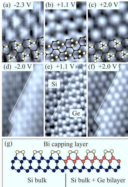
FIG. 1. (Color online) (a)–(c) STM topographs of clean Si(111)-√3×√3-Bi as a function of sample voltage. Tunneling current 0.5 nA, image width 20 Å. (d)–(f) The same for a lateral boundary between clean (Si) and Ge-terminated (Ge) Si(111)-√3×√3-Bi. Image width 40 Å. (g) Schematic side view of the Si-Ge lateral boundary.
