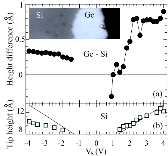
FIG. 2. (a) Apparent height difference between clean (Si) and Ge-terminated (Ge) Si(111)-√3×√3-Bi measured in STM as a function of sample voltage. Tunneling current 0.1 nA. The line represents a guide to the eyes. (b) Corresponding tip height over Si. Tunneling current 0.1 nA. The line represents a tip trajectory for STS measurements [cf. Fig. 3(a)]. Inset: STM topograph of the measurement area. Sample voltage 2.2 V, image width 40 nm.
