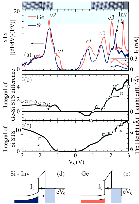
FIG. 3. (Color online) (a) STS measured over clean (Si) and Ge-terminated (Ge) Si(111)- \sqrt{3} \times \sqrt{3} -Bi. Valence band ( v1, v2 ) and conduction band ( c1-c3 ) LDOS features and a bulk inversion ( Inv ) are labeled. Inset: tunneling current change corresponding to the bulk inversion. (b) Line: integral of the difference between Ge STS and Si STS with respect to voltage. Points: the voltage dependence of the STM contrast from Fig. 2(a). (c) Line: integral of the Si STS with respect to voltage. Points: the voltage dependence of the Si tip height from Fig. 2(b). [(d) and (e)] Different positions of Inv in Si and Ge STS indicate a weaker tip-induced band bending in Ge. Under such conditions with increasing V_s , the inversion will be observed first in Si: compare (d) and (e) for the same V_s in Ge and Si.
