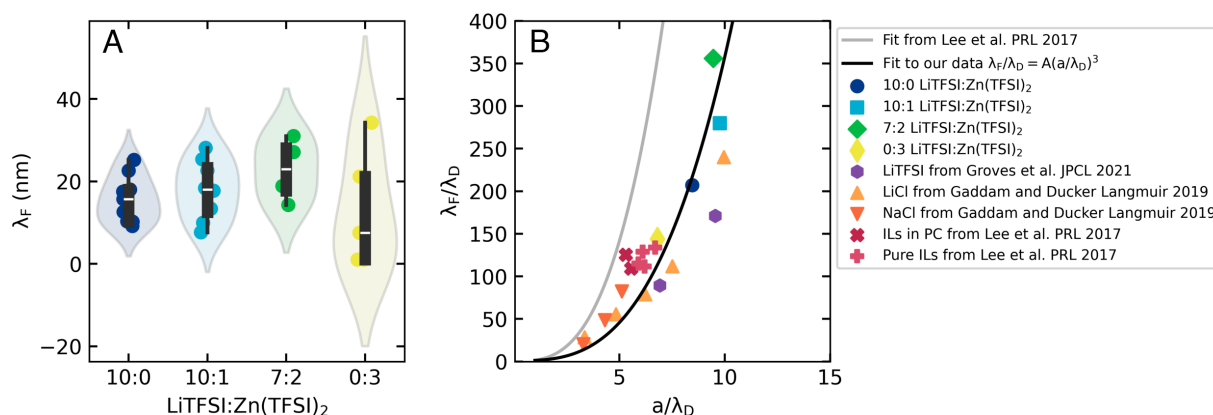
Fig. 6. Decay length scaling analysis. (A) The measured decay length, \lambda_F , for all electrolyte concentrations, in which labels denote molality. (B) Ratio of \lambda_F , over the Debye length, \lambda_D , plotted vs. the average ion diameter, a , also scaled by the \lambda_D . Fit lines are from the Lee et al. (9) scaling analysis and from fitting that cubic relationship to our four electrolytes. Superimposed are data points of other concentrated electrolytes from refs. 9, 11, 13. For our data, a is taken as the cluster spacing from the WAXS measurements in Fig. 1C.
