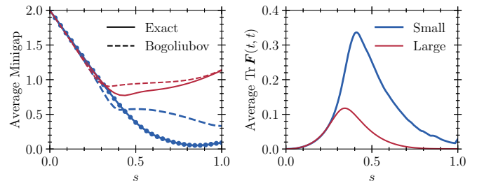
FIG. 13. (Left) Ensemble-averaged minigaps for the two data sets at N = 10 . (Right) Ensemble-averaged sum over the statistical fluctuations for the same parameters as in Fig. 12.
