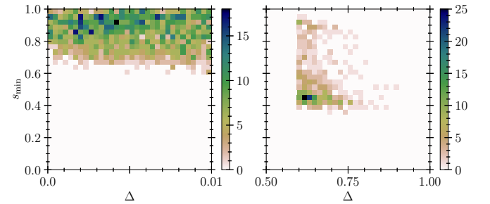
FIG. 20. Minigap size \Delta versus location s_{\min} at N = 12 . The cutoff \Delta_{\text{large}} \sim 0.6 is visible on the right.
