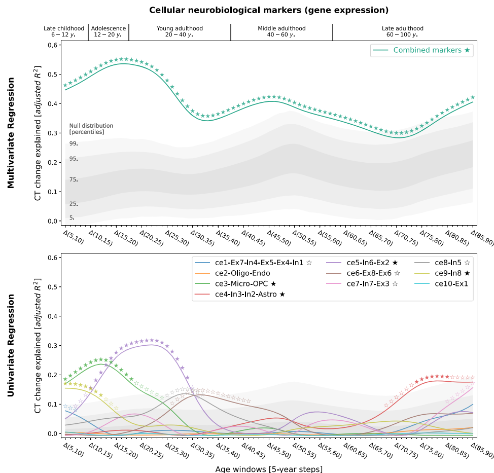
Fig. 4 | Modeled lifespan CT change patterns explained by cellular neurobiological markers. Associations between modeled lifespan CT change and neurobiological markers derived from mRNA expression data. The figure layout and shown plot elements correspond to Fig. 4. See Fig. S6C for all CT change maps, and
