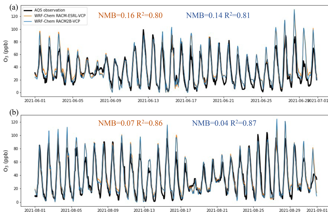
Figure 2. The comparison of time series of hourly \text{O}_3 between AQS and two WRF-Chem simulations, one with RACM-ESRL-VCP and another with the RACM2B-VCP chemical mechanism at the AQS site located at Pasadena ( -118.13, 34.13^\circ ). The corresponding NMB and R^2 between model simulations and observations of hourly \text{O}_3 are shown in each plot.
