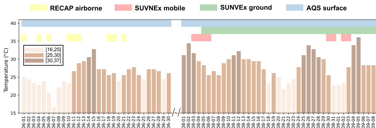
Figure 1. The summary of observations used for WRF-Chem evaluation spanning 1 June to 8 September 2021. It includes 9 d of airborne measurements from the RECAP-CA field campaign in June 2021; 8 d of mobile measurements from the SUVNEx field campaign in August and September 2021; ground site measurements from SUVNEx between 5 August and 8 September 2021; and continuous surface measurements at AQS monitoring sites in June, August, and September 2021. The days are categorized into three groups based on the surface temperature at noon in Pasadena: “low temperature” between 16 to 25 °C, “median temperature” between 25 to 30 °C, and “high temperature” between 30 to 37 °C.
