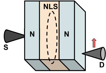
FIG. 14. Proposed setup for the detection of the spatial current profile: a STM tip or a quantum point contact on one surface of the metallic sample (S) acts as a point source of electrons. After passing through the NLS slab, the current acquires an intensity distribution as a function of the distance from the axis, which can be probed by a mobile STM tip (D) on the other surface.
