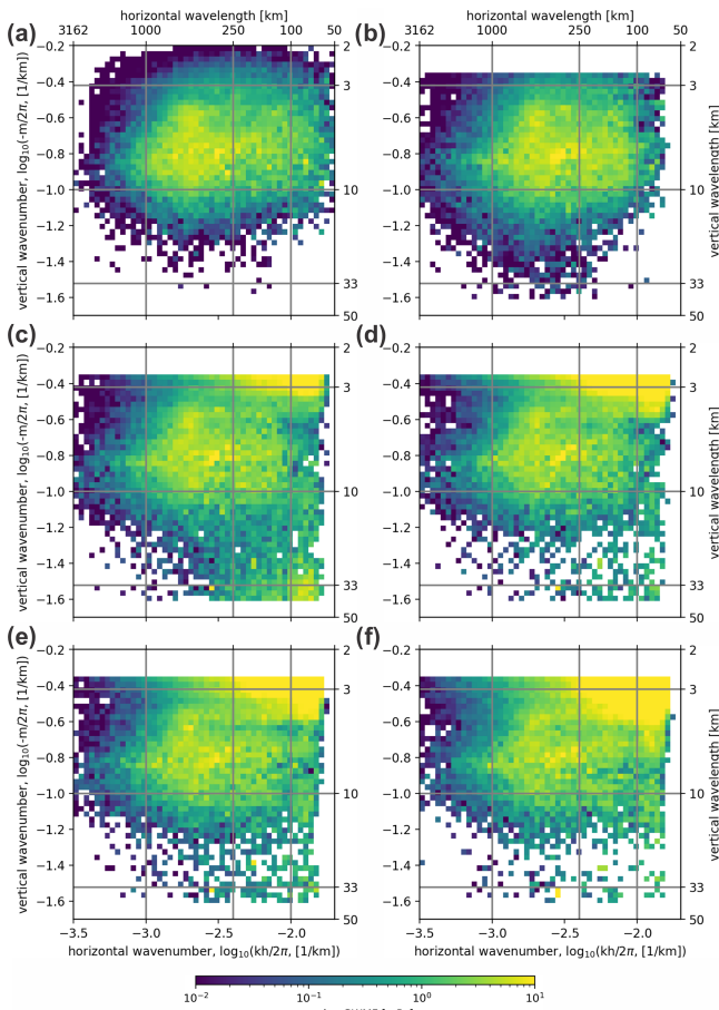
Figure 4. Comparison of averaged spectra for 80° S to 80° N and all longitudes for 3 January 2006 at 25 km altitude as derived via the S3D cascade. Panel (a) shows the spectrum of the NWP data on the original grid; panel (b) the data for the orbit-sampled NWP; and panels (c)–(f) the simulated retrievals for different noise levels of (c) goal, (d) threshold, (e) 2 times the goal, and (f) 3 times the goal.
