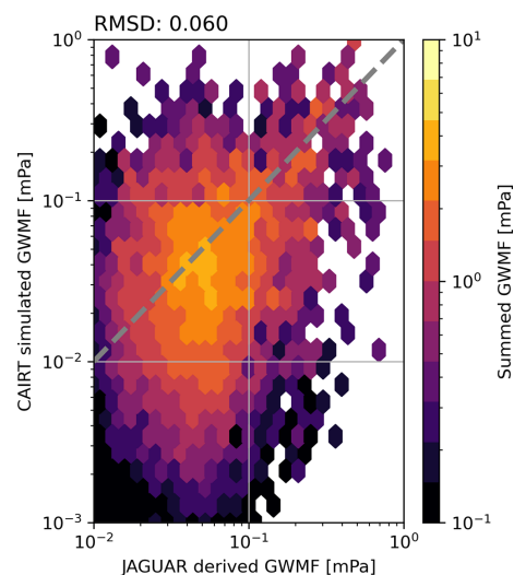
Figure B3. Scatter distribution of GWMF estimated from JAGUAR (horizontal axis) and CAIRT simulations (vertical axis) at 70 km (shown in Fig. 17). Color shading shows the summed GWMF in the respective bin. Note the logarithmic scale.
