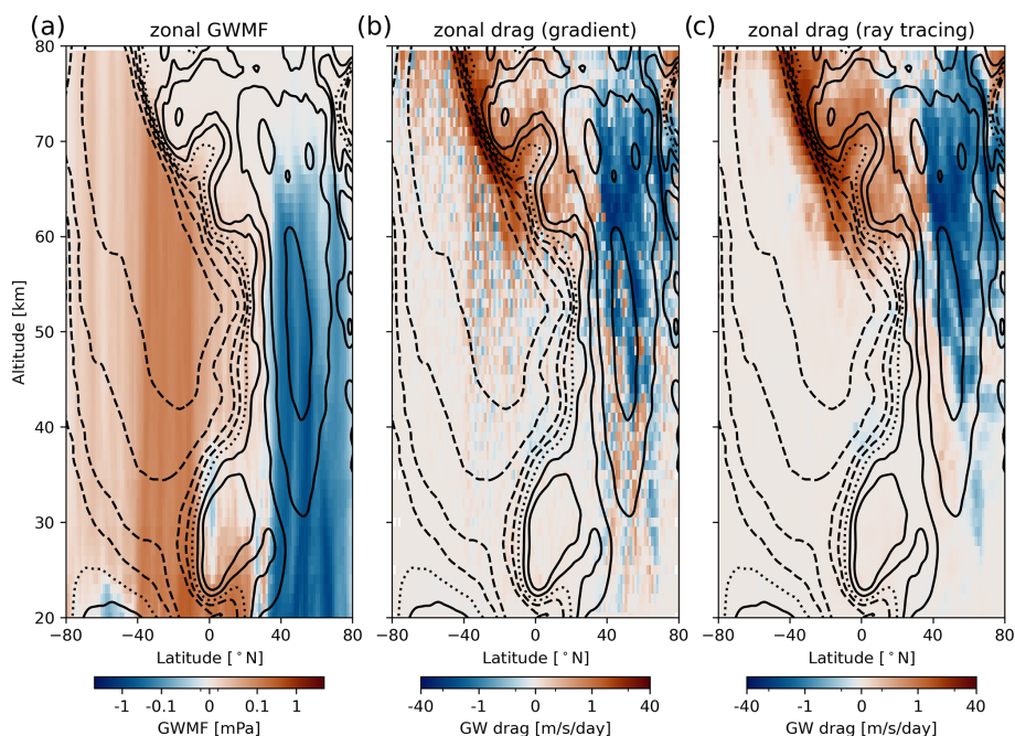
Figure 19. Zonal-mean zonal GWMF (a) and drag (b, c) as estimated from the ray-tracing experiment. Panels (b) and (c) show the GW drag estimated as the vertical derivative of the GWMF distribution and directly taken from the ray tracer, respectively. The situation and wind profile are the same as in Fig. 16.
