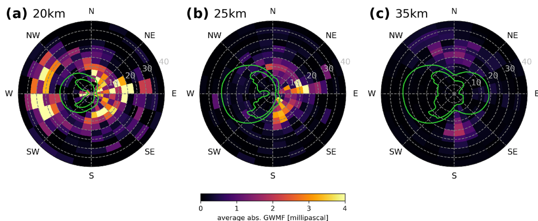
Figure 14. Phase speed diagrams from simulated CAIRT observations and their QBO interactions for the tropics ( 5^{\circ} S to 5^{\circ} N) at (a) 20 km, (b) 25 km, and (c) 35 km altitude. Plotted on top in green are the 50 % and 90 % blocking likelihood (outer and inner line, respectively). The analysis is performed on a snapshot of 11 January 2006.
