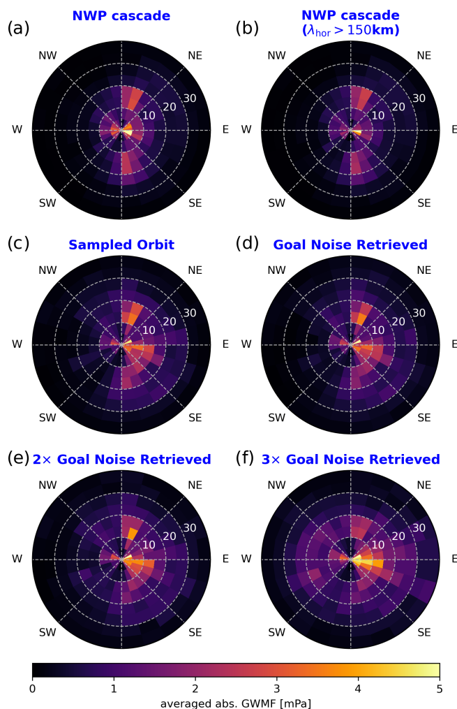
Figure 7. Comparison of averaged phase speed spectra for 80° S to 80° N and all longitudes for NWP data of 3 January 2006 analyzed by an S3D cascade (a), the same data but limited to horizontal wavelengths of 150 km and longer (b), data sampled onto CAIRT grid (c), and end-to-end simulated retrievals with various noise levels (d–f).
