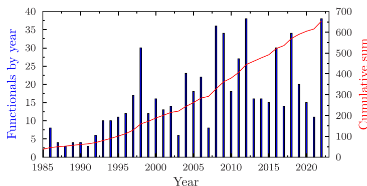
Figure 2. Statistics on the number of functionals by year of (latest) publication and the cumulative number of functionals based on the functionals implemented in Libxc version 6.2.0 [18].
