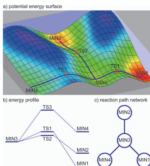
Figure 8. (a) A schematic of a two-dimensional PES, (b) an energy profile representation of (a), and (c) a reaction path network representation of (a). MINs and TSs correspond to local minima and transition states, respectively.
