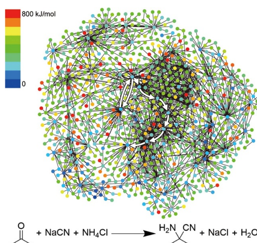
Figure 9. An example illustrating how complex a network describing a chemical reaction can be, even for a simple organic reaction, in this case the condensation step of the Strecker amino acid synthesis indicated in the chemical equation. Nodes and edges represent different chemical species and elementary steps, respectively. The network comprehensively includes not only the most feasible route to the major product, \alpha -aminonitrile, highlighted by the white arrows, but also minor paths that cross the boundary between kinetically accessible and inaccessible regions from reactant's node, thus proving that the reaction yields \alpha -aminonitrile. Reproduced from [184]. CC BY 4.0.
