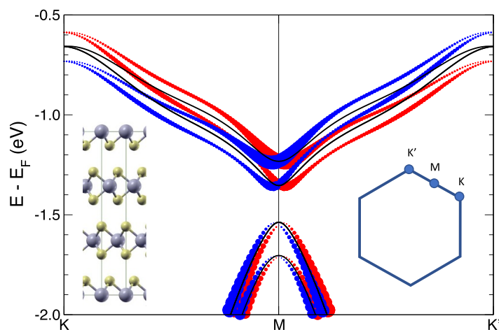
Figure 5. Spin–orbit splitting of the valence bands in 3R-MoS 2 : black lines show the band structure without spin–orbit coupling (SOC), red/blue dots indicate the spin polarization perpendicular to the layers (up/down) of the bands with SOC included. Insets show the structure (grey/yellow spheres: Mo/S) and the Brillouin zone.
