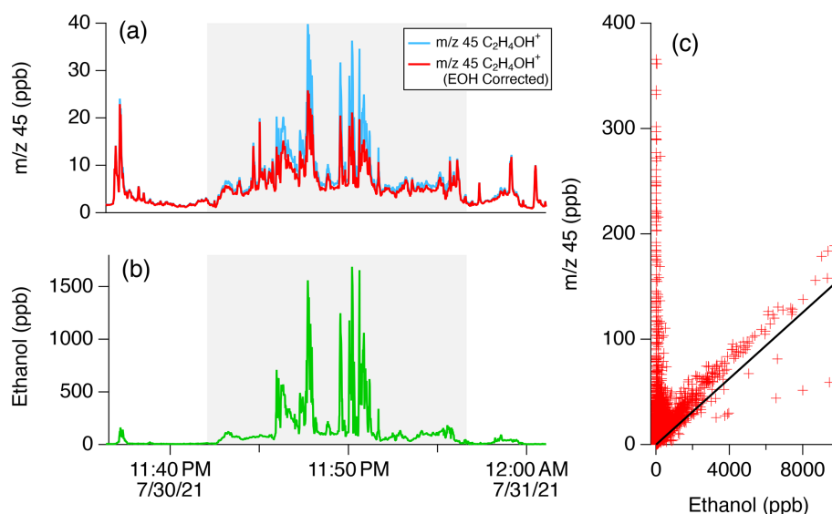
Figure 11. Demonstration of the impacts of ethanol on mobile drive data in downtown Las Vegas during the evening drive on 30 July. (a) Time series of the signal at m/z 45 ( \text{C}_2\text{H}_4\text{OH}^+ ) with and without the subtraction of the ethanol interference. (b) Time series of ethanol ( m/z 47, \text{C}_2\text{H}_6\text{OH}^+ ). The shaded regions show when the mobile laboratory was sampling along the Las Vegas Strip. (c) Correlation plot of mobile drive data for the entire Las Vegas dataset. The solid line shows the fragmentation ratio of m/z 45 to m/z 47 for ethanol, as derived from the GC-PTR-ToF-MS data (Fig. 10).
