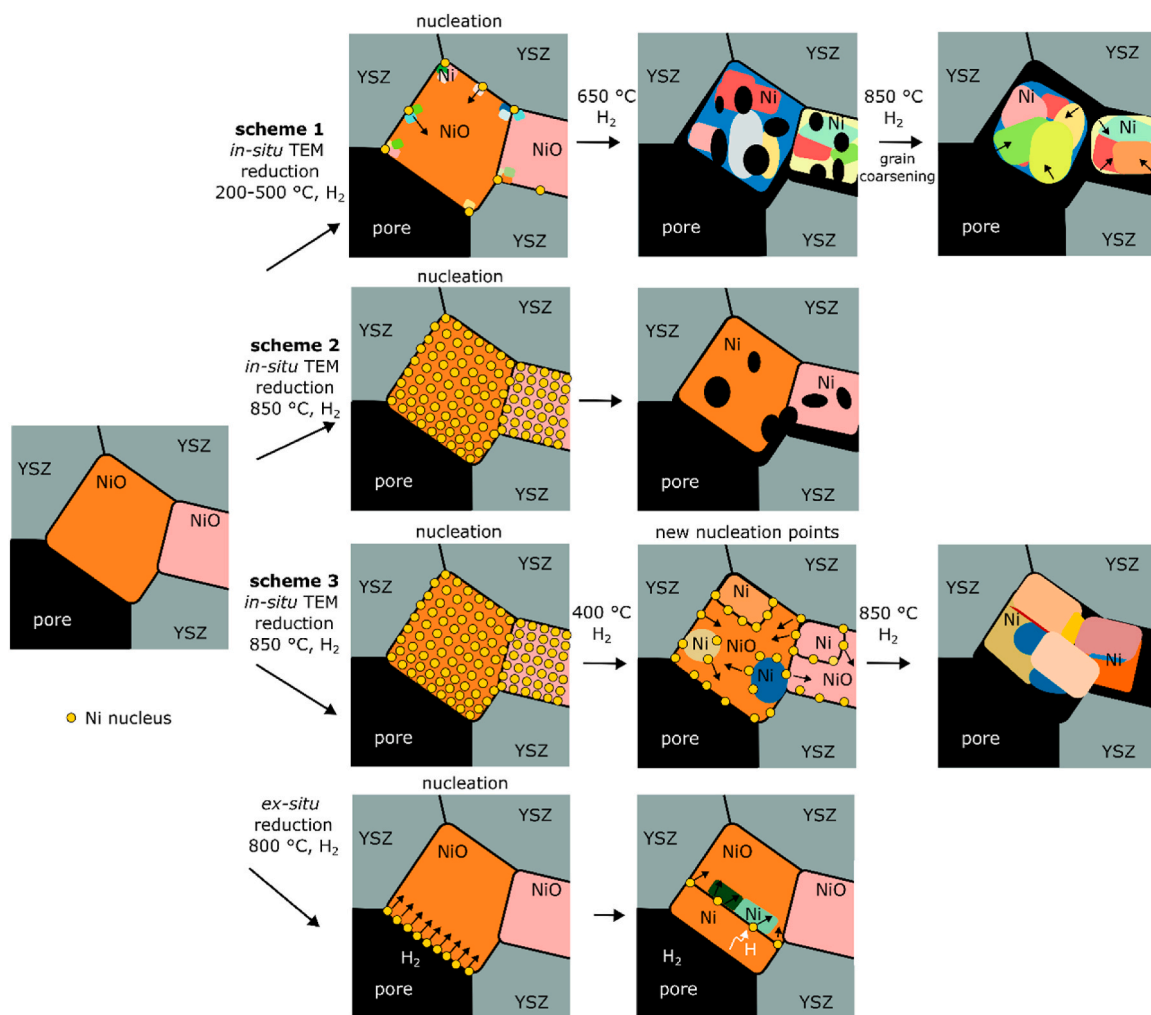
Fig. 7. A sketch of the NiO/YSZ reduction mechanisms taking place during three reduction schemes carried out with the in-situ TEM, compared to the ex-situ reduction of the bulk NiO/YSZ mechanism at high temperatures.
