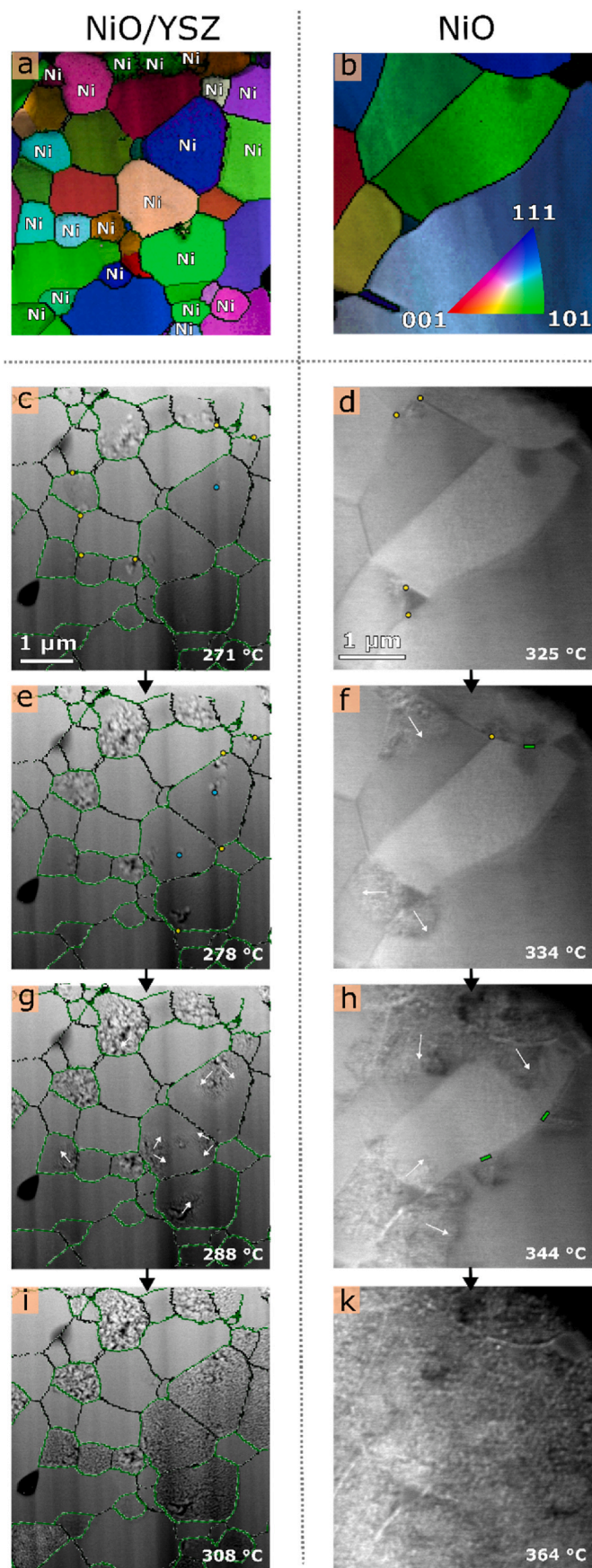
Fig. 2. Reduction of NiO/YSZ and pure Ni. a. Grain orientation in NiO/YSZ cermet before the reduction in H_2 . b. Grain orientation in pure NiO before the reduction in H_2 . Both a and b are mapped with ASTAR precession electron diffraction. Dimensions of images a and b are the same as on c and d, correspondingly. c, e, g, i. HAADF STEM image series taken at different temperatures and 27 kPa H_2 pressure during in-situ reduction of NiO/YSZ. The phase boundaries between NiO_x and YSZ are marked with dark green and grain boundaries between NiO_x/NiO_x or YSZ/YSZ are marked with black lines. d, f, h, k. ADF STEM image series taken at different temperatures and 27 kPa H_2 pressure during in-situ reduction of pure NiO in the presence of 27 kPa H_2 . Yellow dots indicate the start of NiO reduction at the triple junctions between NiO and YSZ grains, or NiO/NiO grains in case of pure Ni. Light green lines indicate the start of reduction at grain boundaries in case of pure NiO. Blue dots mark another starting point of NiO reduction: middle of NiO grain (possibly, crystalline defects or FIB artefact induced site). White arrows indicate the direction of the reduction front.
