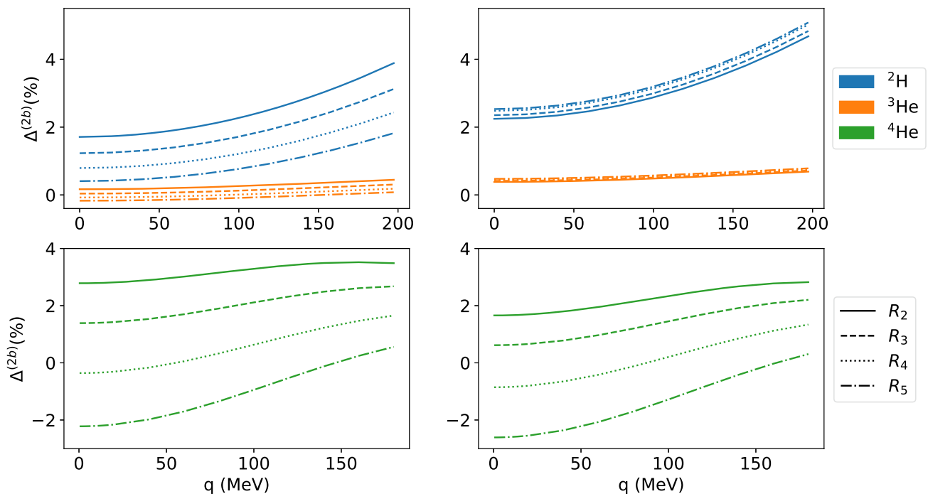
Fig. 4 The percentage relative contribution of two-body corrections of ^2\text{H} , ^3\text{He} , and ^4\text{He} as a function of transfer momentum q for various cut-offs for \text{N}^2\text{LO} (left) and \text{N}^4\text{LO} (right) chiral wave functions
