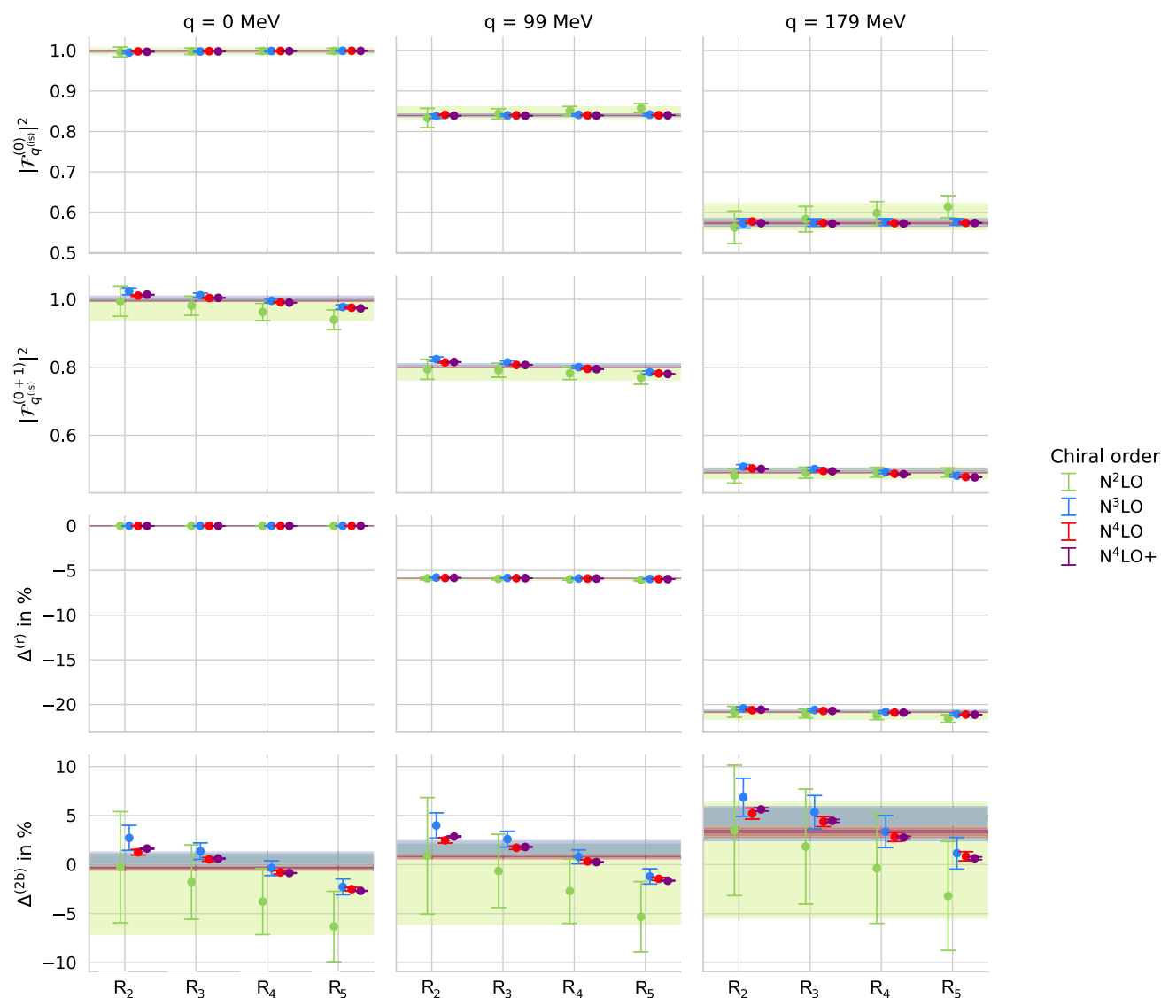
Fig. 6 Isoscalar structure functions of {}^4\text{He} up to chiral order \nu = 0 + 1 as a function of cut-offs for different transfer momentum q . The first and second panel indicate the leading order ( \nu = 0 ) one-nucleon isoscalar structure functions and the full order ( \nu = 0 + 1 ) isoscalar structure
