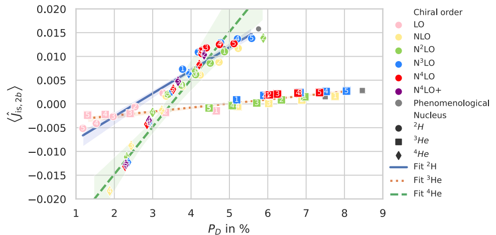
Fig. 7 The plots shows the correlation between the isoscalar structure functions and the D -wave probability for {}^2\text{H} , {}^3\text{He} , and {}^4\text{He} represented by circle, square, and diamond data points. The data points are assigned different colors corresponding to the chiral order of the wave function. The cut-off R_1 used for the calculation is indicated by label i on the data point. For {}^2\text{H} and {}^3\text{He} , we have included the cut-off R_1 = 0.8 fm and results from phenomenological wave functions from Ref. [15]
