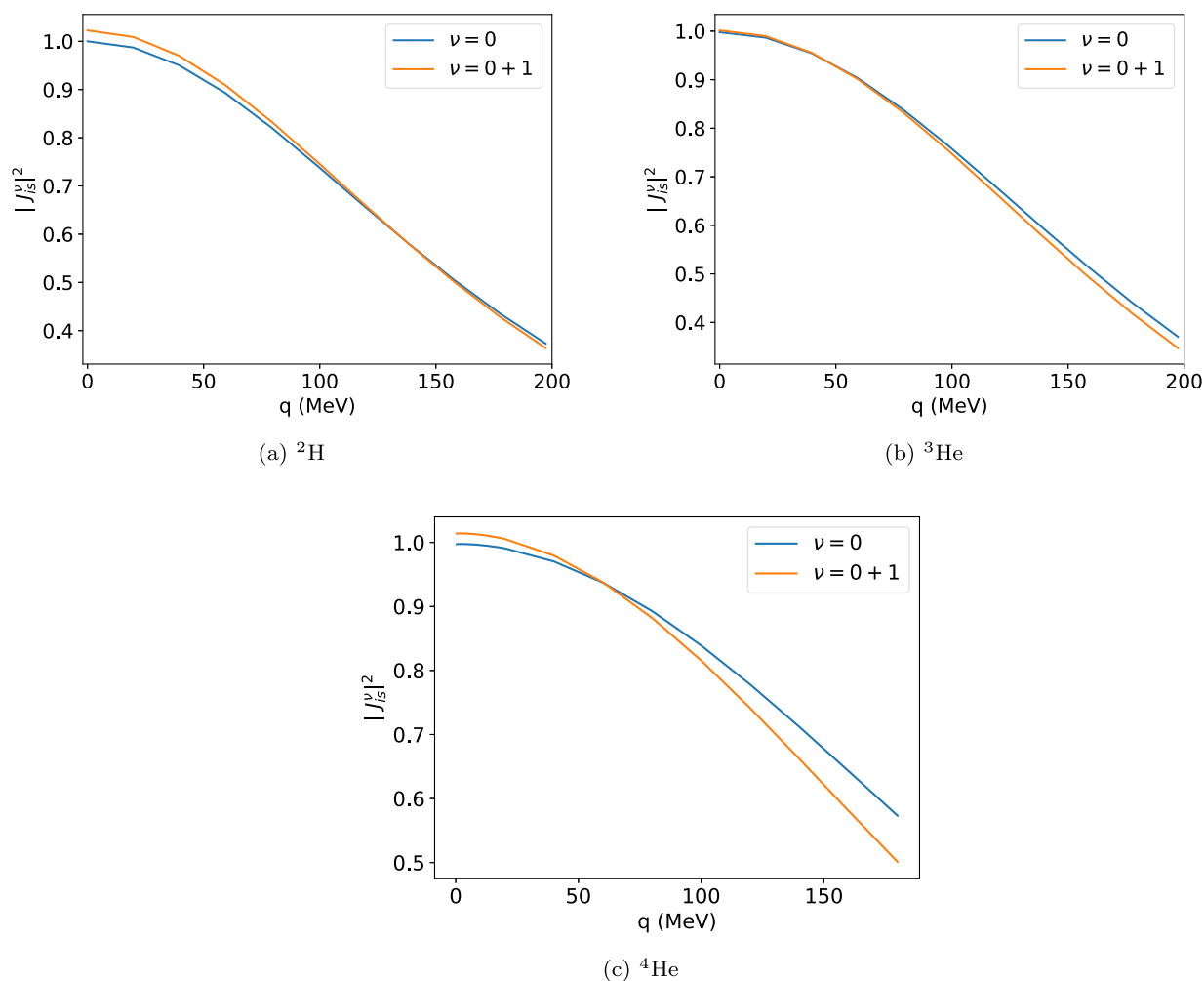
Fig. 2 Isoscalar structure functions of ^2\text{H} , ^3\text{He} , and ^4\text{He} as a function of transfer momentum q . We apply \text{N}^4\text{LO} wave functions with a fixed cut-off R_2 = 0.9 fm. The chiral order \nu = 0 ( 0 + 1 ) is shown by the blue (orange) line
