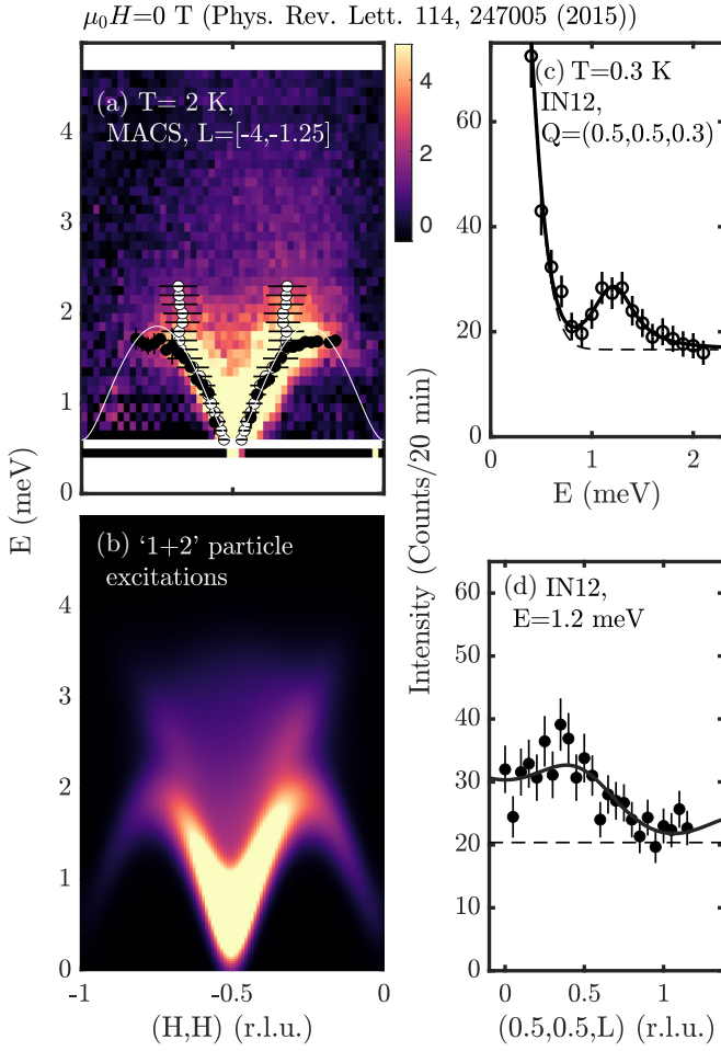
FIG. 2. A summary of the zero field magnetic fluctuations in \text{CeRhIn}_5 below T_N previously reported based on neutron spectroscopy. (a) Neutron spectroscopy measurements on MACS compared against a (b) heuristic multimagnon calculation. A second gapped mode is found in (c) using IN12 which corresponds to fluctuations polarized along the crystallographic c axis as confirmed from a scan of the intensity along [001] shown in (d).
